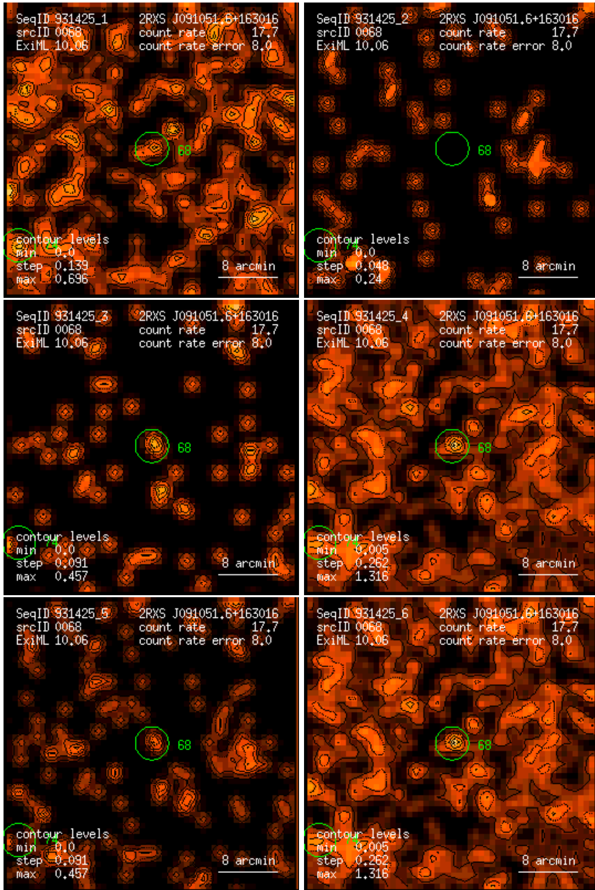
Figure 68: RASS 931425: detection 0068: band rate images, Gaussian filter: (1) PSPC channels 11 – 41, (2) 52 – 90, (3) 91 – 201, (4) 11 – 235, (5) 52 – 201, (6) 11 – 201. Broad band rates in counts/ks. Band rate contour levels in counts/ks/arcmin 2 .
