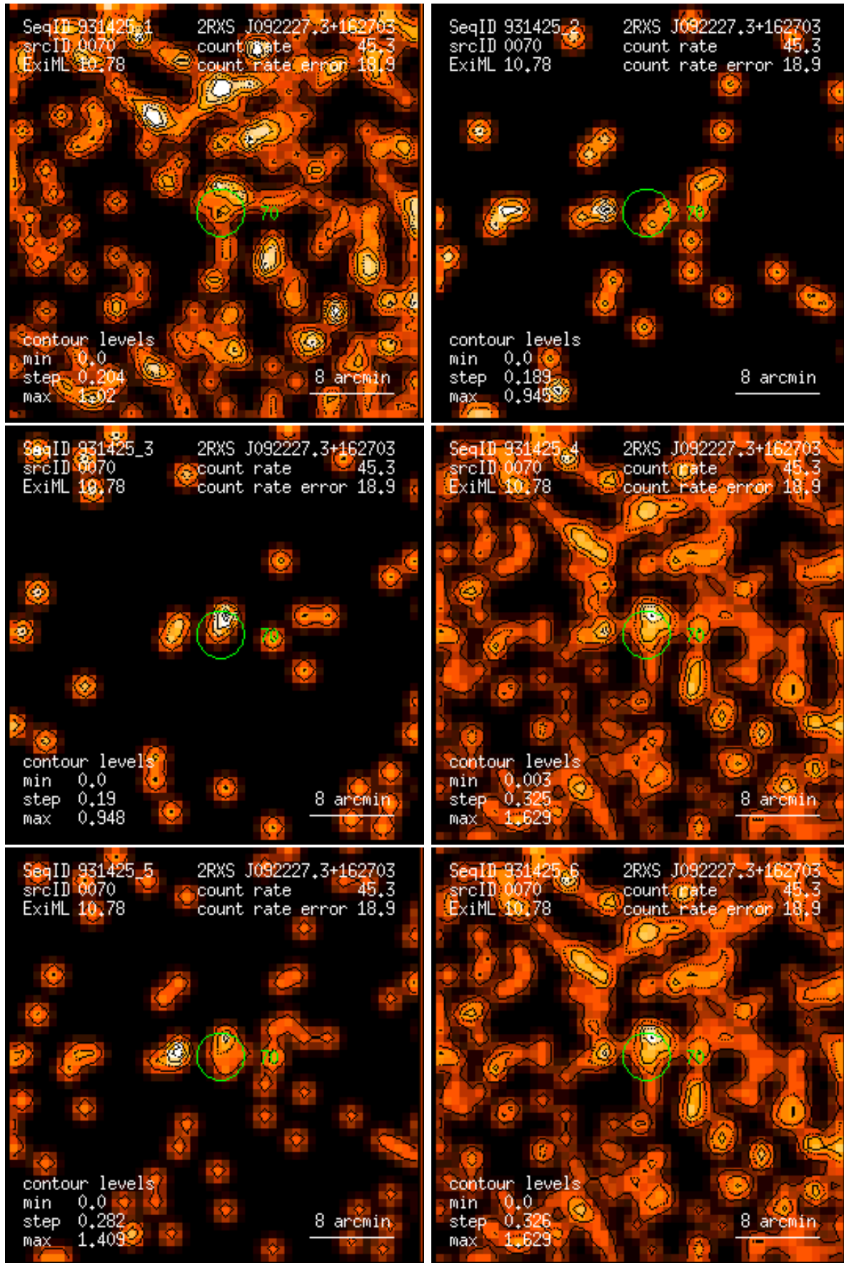
Figure 70: RASS 931425: detection 0070: band rate images, Gaussian filter: (1) PSPC channels 11 – 41, (2) 52 – 90, (3) 91 – 201, (4) 11 – 235, (5) 52 – 201, (6) 11 – 201. Broad band rates in counts/ks. Band rate contour levels in counts/ks/arcmin 2 .
