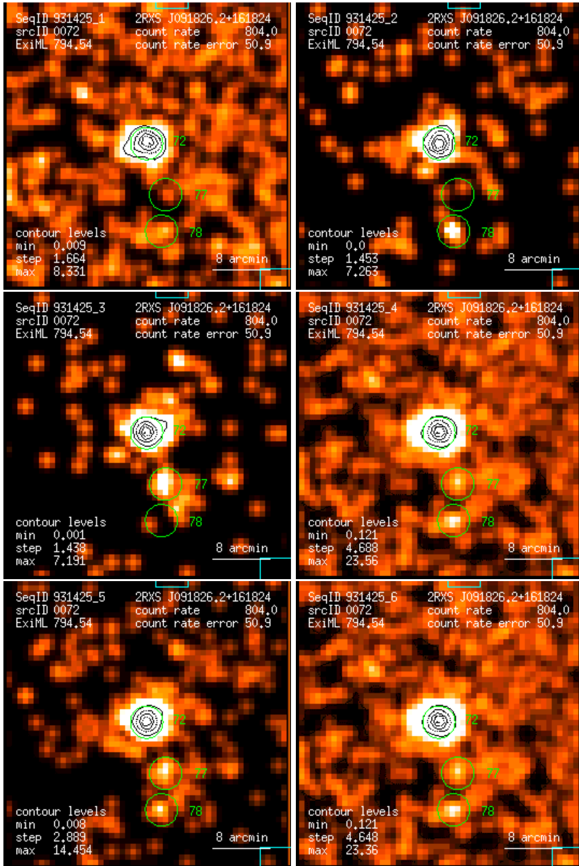
Figure 72: RASS 931425: detection 0072: band rate images, Gaussian filter: (1) PSPC channels 11 – 41, (2) 52 – 90, (3) 91 – 201, (4) 11 – 235, (5) 52 – 201, (6) 11 – 201. Broad band rates in counts/ks. Band rate contour levels in counts/ks/arcmin 2 .
