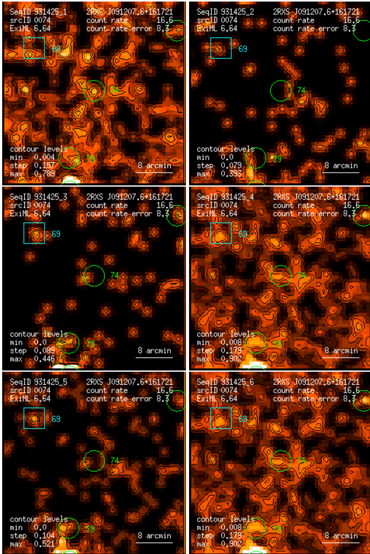
Figure 74: RASS 931425: detection 0074: band rate images, Gaussian filter: (1) PSPC channels 11 – 41, (2) 52 – 90, (3) 91 – 201, (4) 11 – 235, (5) 52 – 201, (6) 11 – 201. Broad band rates in counts/ks. Band rate contour levels in counts/ks/arcmin 2 .
