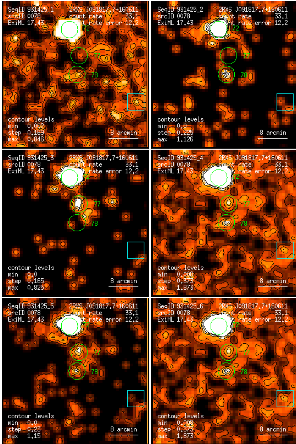
Figure 78: RASS 931425: detection 0078: band rate images, Gaussian filter: (1) PSPC channels 11 – 41, (2) 52 – 90, (3) 91 – 201, (4) 11 – 235, (5) 52 – 201, (6) 11 – 201. Broad band rates in counts/ks. Band rate contour levels in counts/ks/arcmin 2 .
