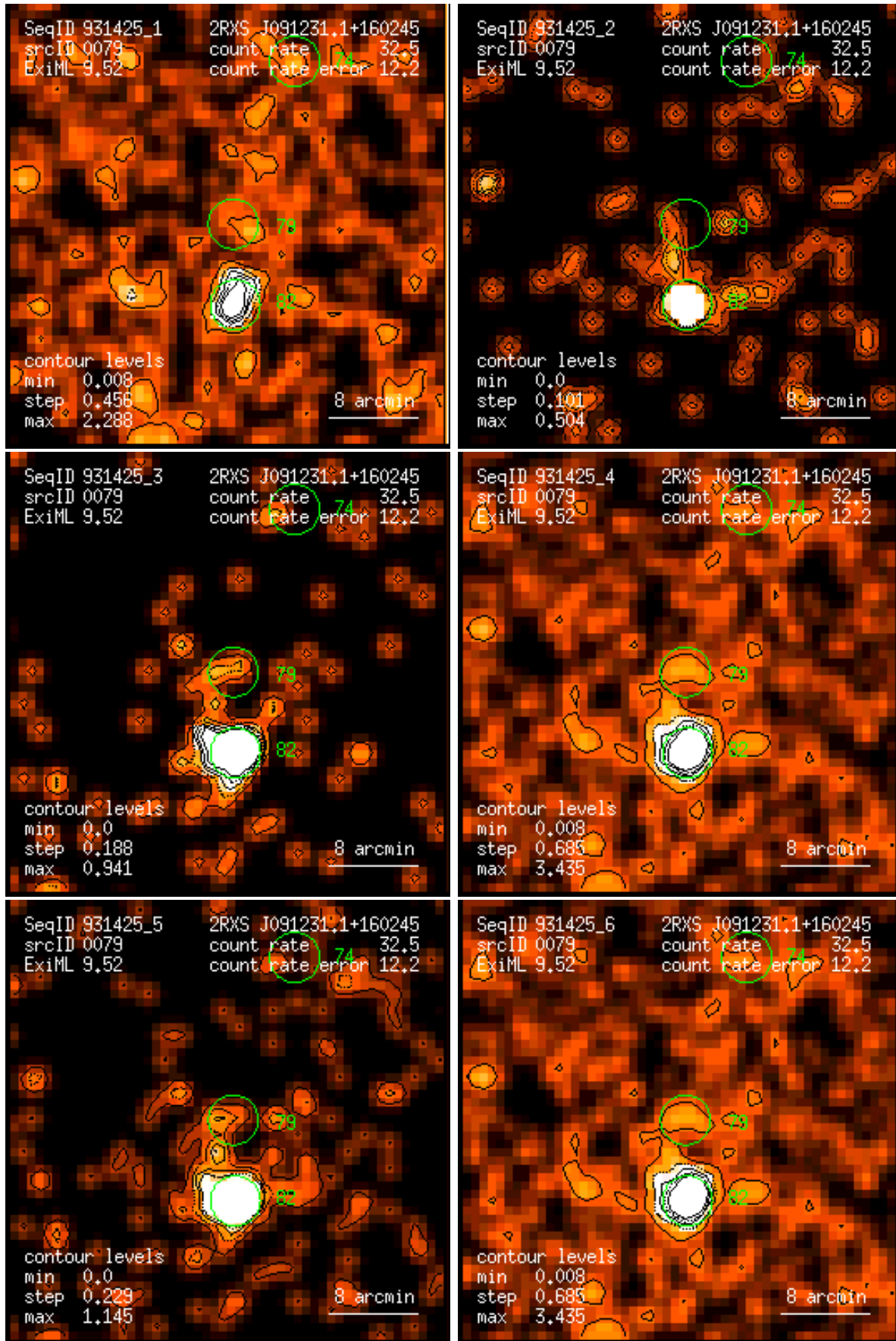
Figure 79: RASS 931425: detection 0079: band rate images, Gaussian filter: (1) PSPC channels 11 – 41, (2) 52 – 90, (3) 91 – 201, (4) 11 – 235, (5) 52 – 201, (6) 11 – 201. Broad band rates in counts/ks. Band rate contour levels in counts/ks/arcmin 2 .
