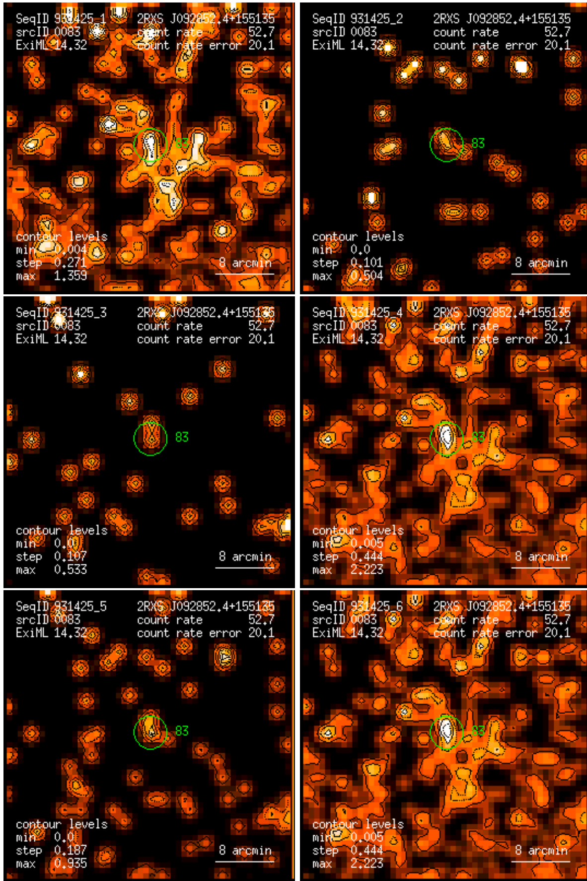
Figure 83: RASS 931425: detection 0083: band rate images, Gaussian filter: (1) PSPC channels 11 – 41, (2) 52 – 90, (3) 91 – 201, (4) 11 – 235, (5) 52 – 201, (6) 11 – 201. Broad band rates in counts/ks. Band rate contour levels in counts/ks/arcmin 2 .
