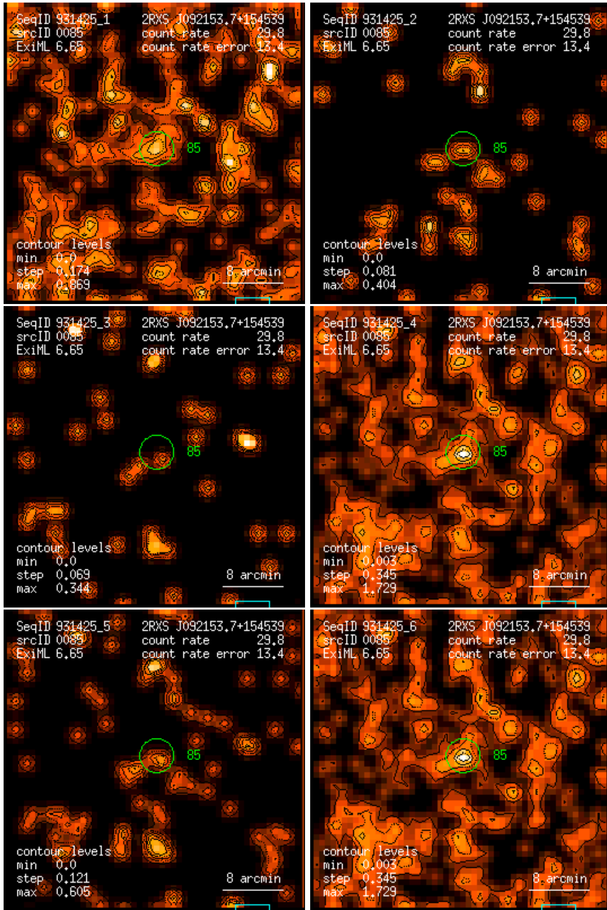
Figure 85: RASS 931425: detection 0085: band rate images, Gaussian filter: (1) PSPC channels 11 – 41, (2) 52 – 90, (3) 91 – 201, (4) 11 – 235, (5) 52 – 201, (6) 11 – 201. Broad band rates in counts/ks. Band rate contour levels in counts/ks/arcmin 2 .
