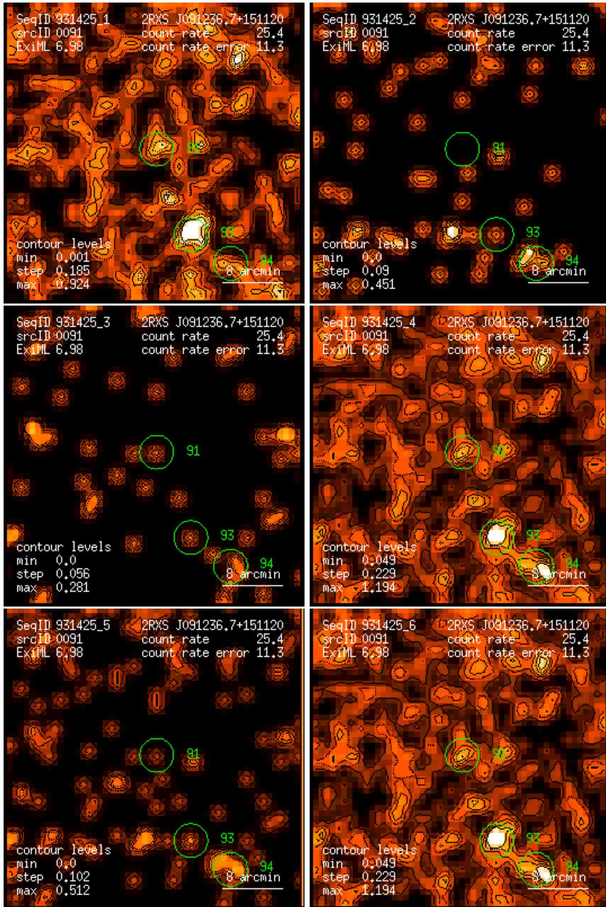
Figure 91: RASS 931425: detection 0091: band rate images, Gaussian filter: (1) PSPC channels 11 – 41, (2) 52 – 90, (3) 91 – 201, (4) 11 – 235, (5) 52 – 201, (6) 11 – 201. Broad band rates in counts/ks. Band rate contour levels in counts/ks/arcmin 2 .
