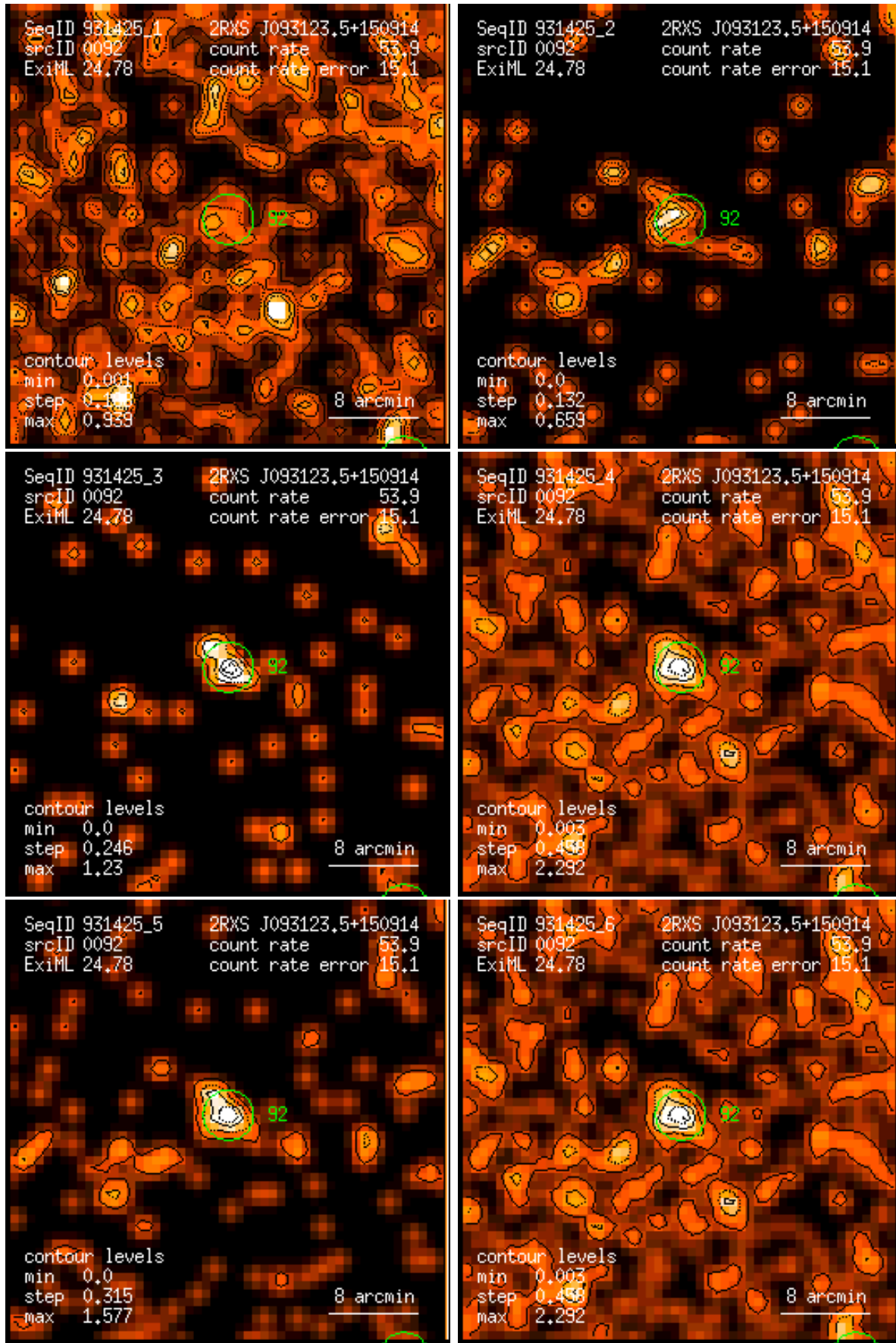
Figure 92: RASS 931425: detection 0092: band rate images, Gaussian filter: (1) PSPC channels 11 – 41, (2) 52 – 90, (3) 91 – 201, (4) 11 – 235, (5) 52 – 201, (6) 11 – 201. Broad band rates in counts/ks. Band rate contour levels in counts/ks/arcmin 2 .
