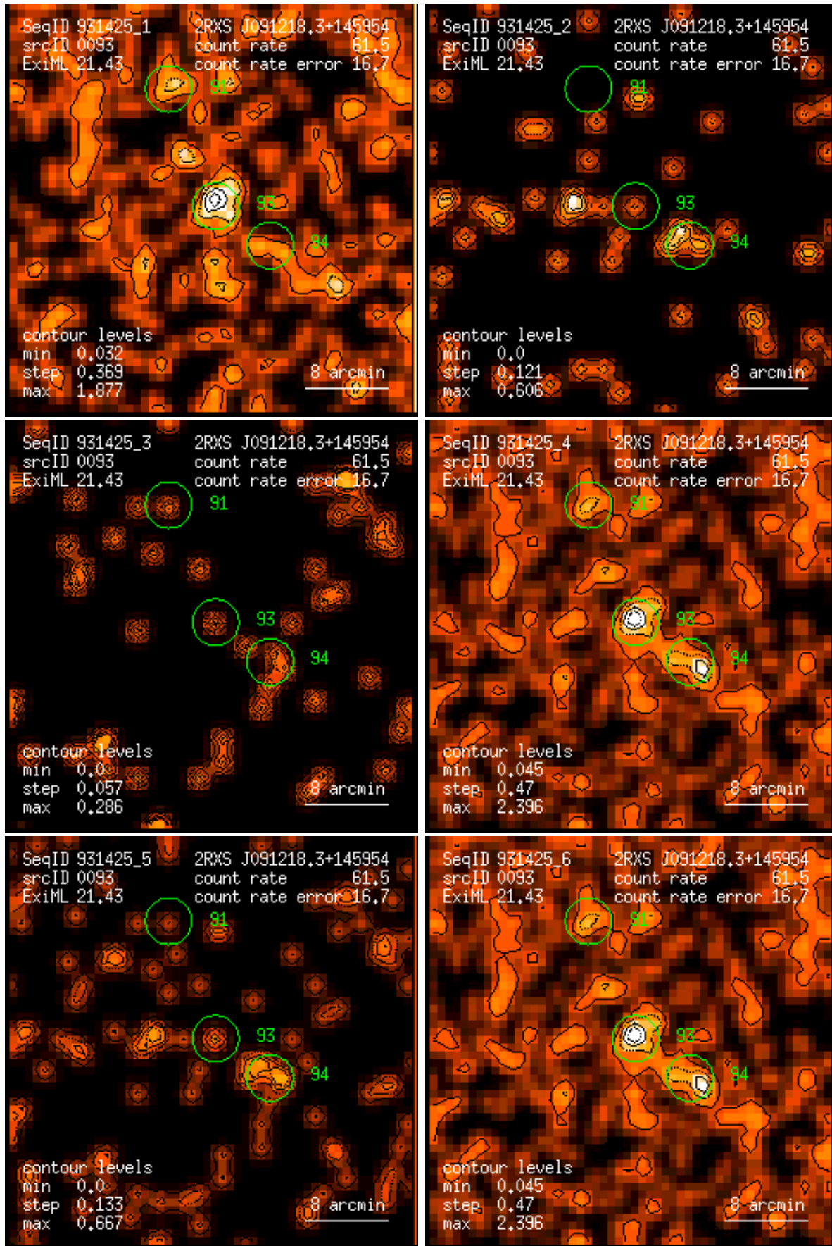
Figure 93: RASS 931425: detection 0093: band rate images, Gaussian filter: (1) PSPC channels 11 – 41, (2) 52 – 90, (3) 91 – 201, (4) 11 – 235, (5) 52 – 201, (6) 11 – 201. Broad band rates in counts/ks. Band rate contour levels in counts/ks/arcmin 2 .
