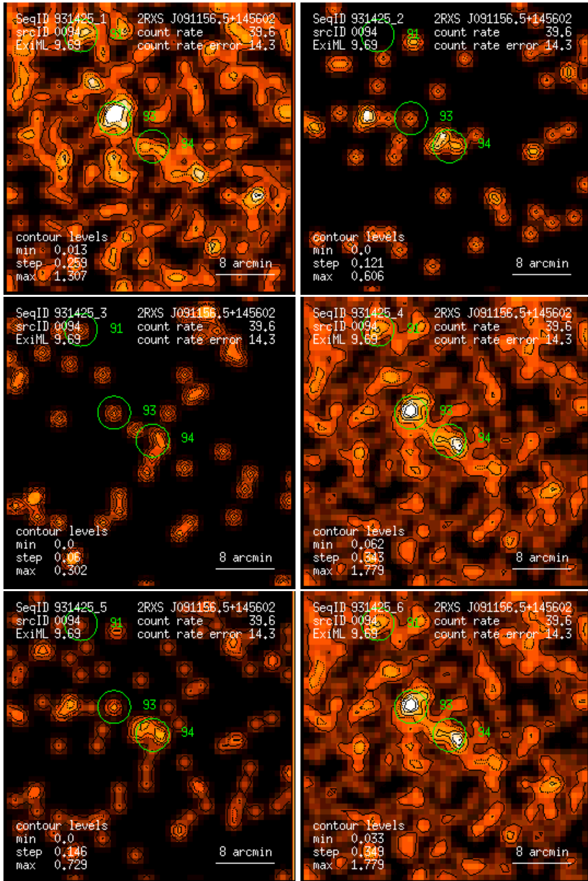
Figure 94: RASS 931425: detection 0094: band rate images, Gaussian filter: (1) PSPC channels 11 – 41, (2) 52 – 90, (3) 91 – 201, (4) 11 – 235, (5) 52 – 201, (6) 11 – 201. Broad band rates in counts/ks. Band rate contour levels in counts/ks/arcmin 2 .
