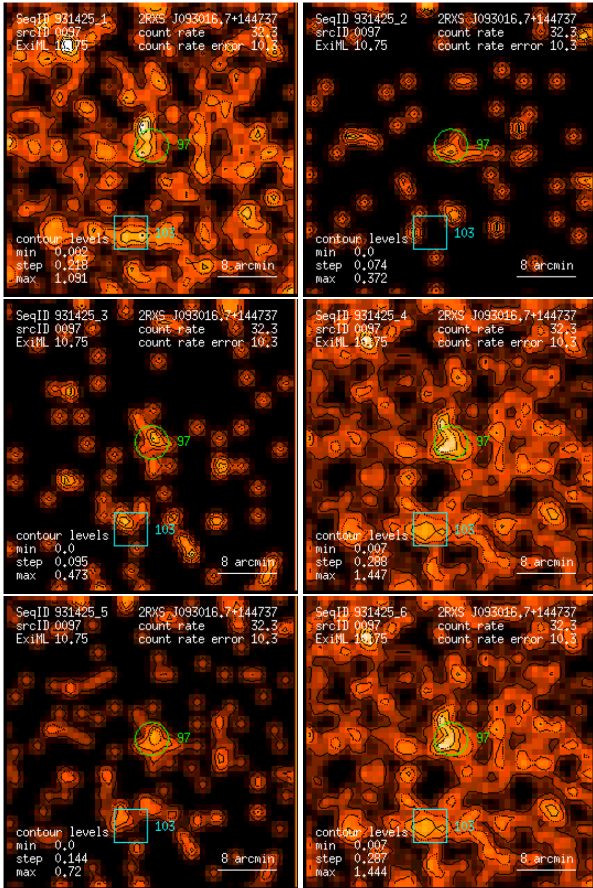
Figure 97: RASS 931425: detection 0097: band rate images, Gaussian filter: (1) PSPC channels 11 – 41, (2) 52 – 90, (3) 91 – 201, (4) 11 – 235, (5) 52 – 201, (6) 11 – 201. Broad band rates in counts/ks. Band rate contour levels in counts/ks/arcmin 2 .
