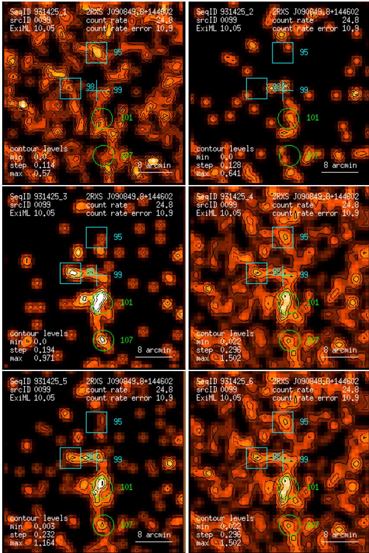
Figure 99: RASS 931425: detection 0099: band rate images, Gaussian filter: (1) PSPC channels 11 – 41, (2) 52 – 90, (3) 91 – 201, (4) 11 – 235, (5) 52 – 201, (6) 11 – 201. Broad band rates in counts/ks. Band rate contour levels in counts/ks/arcmin 2 .
