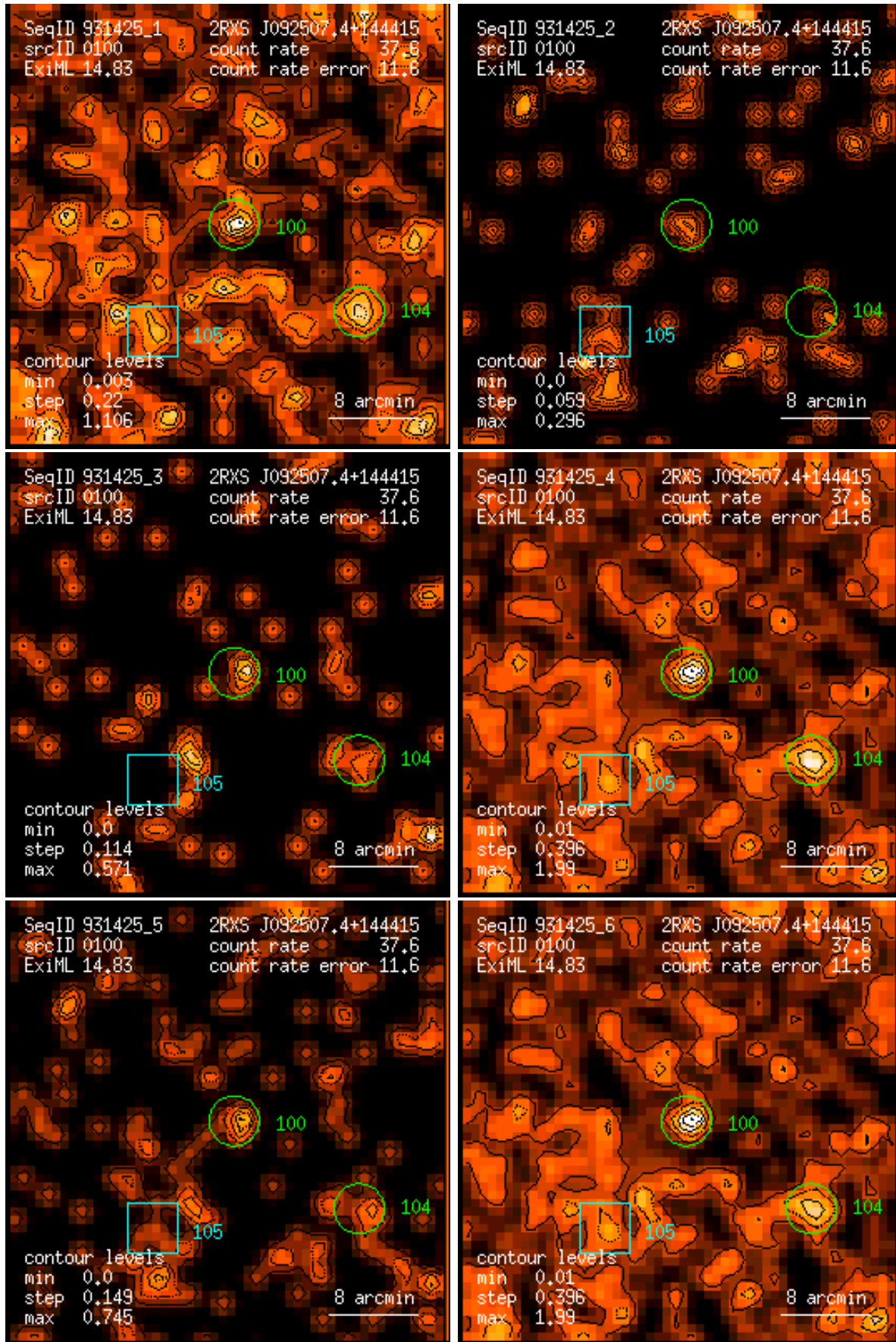
Figure 100: RASS 931425: detection 0100: band rate images, Gaussian filter: (1) PSPC channels 11 – 41, (2) 52 – 90, (3) 91 – 201, (4) 11 – 235, (5) 52 – 201, (6) 11 – 201. Broad band rates in counts/ks. Band rate contour levels in counts/ks/arcmin 2 .
