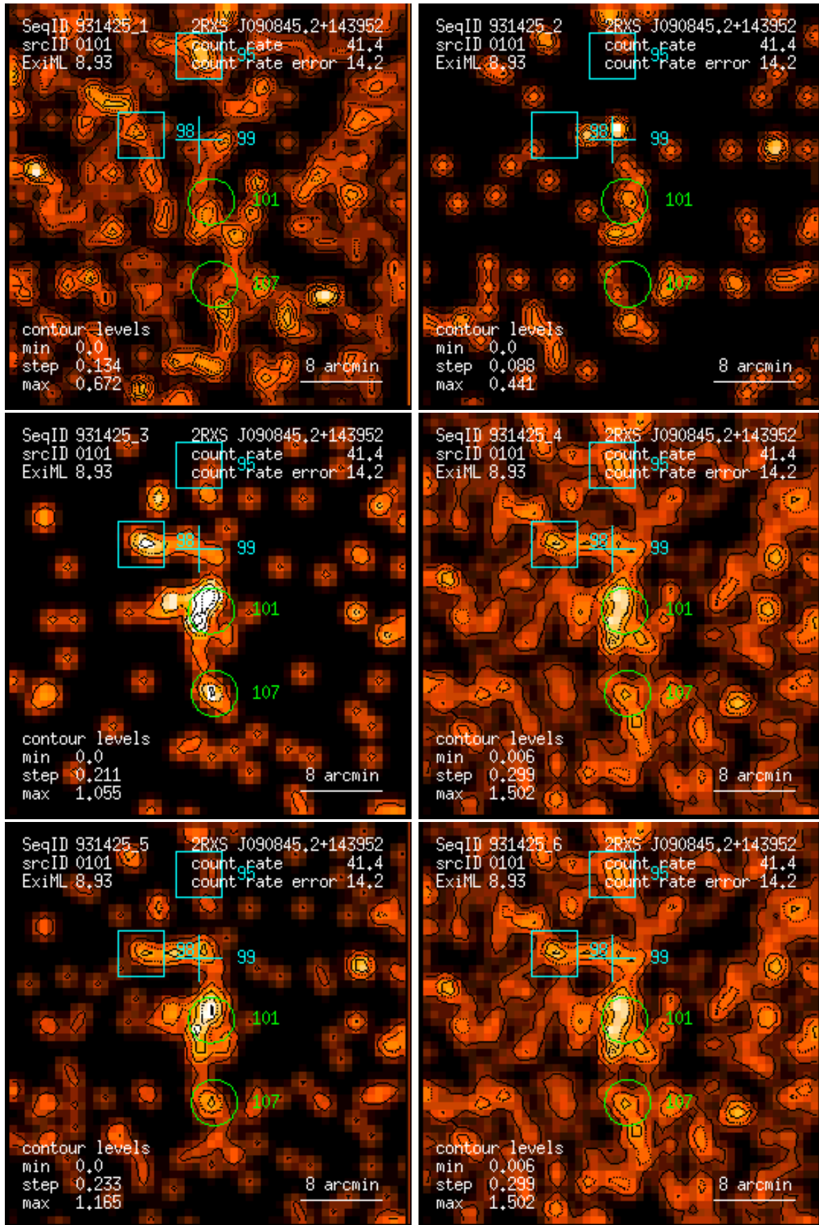
Figure 101: RASS 931425: detection 0101: band rate images, Gaussian filter: (1) PSPC channels 11 – 41, (2) 52 – 90, (3) 91 – 201, (4) 11 – 235, (5) 52 – 201, (6) 11 – 201. Broad band rates in counts/ks. Band rate contour levels in counts/ks/arcmin 2 .
