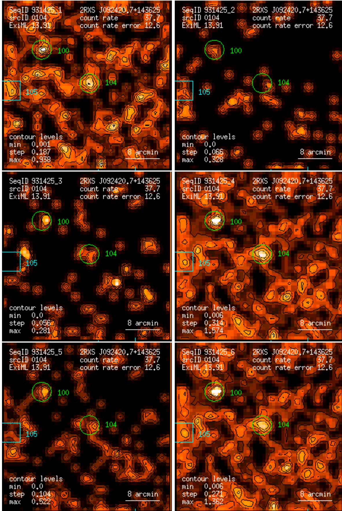
Figure 104: RASS 931425: detection 0104: band rate images, Gaussian filter: (1) PSPC channels 11 – 41, (2) 52 – 90, (3) 91 – 201, (4) 11 – 235, (5) 52 – 201, (6) 11 – 201. Broad band rates in counts/ks. Band rate contour levels in counts/ks/arcmin 2 .
