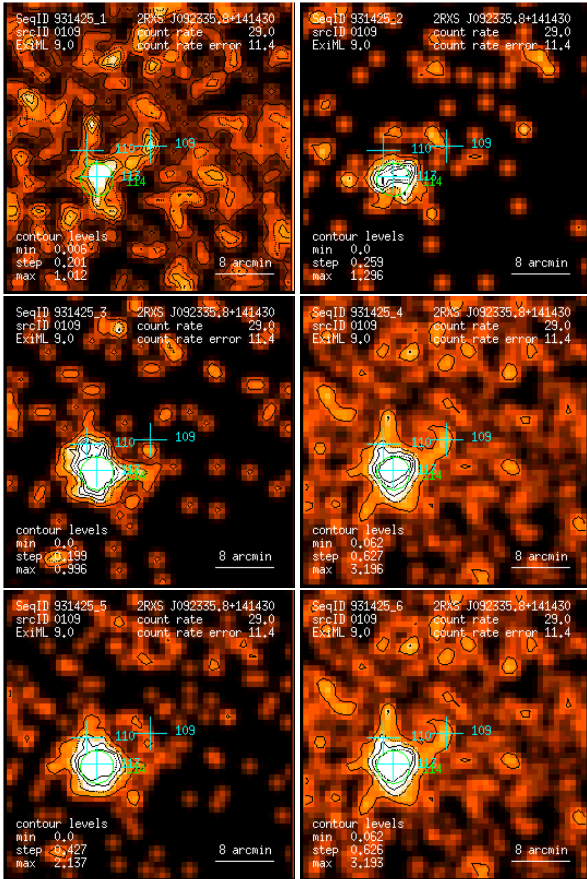
Figure 109: RASS 931425: detection 0109: band rate images, Gaussian filter: (1) PSPC channels 11 – 41, (2) 52 – 90, (3) 91 – 201, (4) 11 – 235, (5) 52 – 201, (6) 11 – 201. Broad band rates in counts/ks. Band rate contour levels in counts/ks/arcmin 2 .
