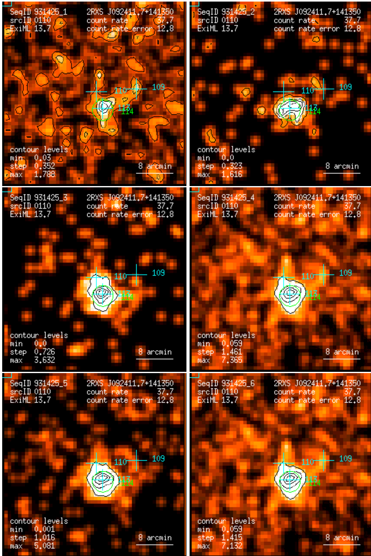
Figure 110: RASS 931425: detection 0110: band rate images, Gaussian filter: (1) PSPC channels 11 – 41, (2) 52 – 90, (3) 91 – 201, (4) 11 – 235, (5) 52 – 201, (6) 11 – 201. Broad band rates in counts/ks. Band rate contour levels in counts/ks/arcmin 2 .
