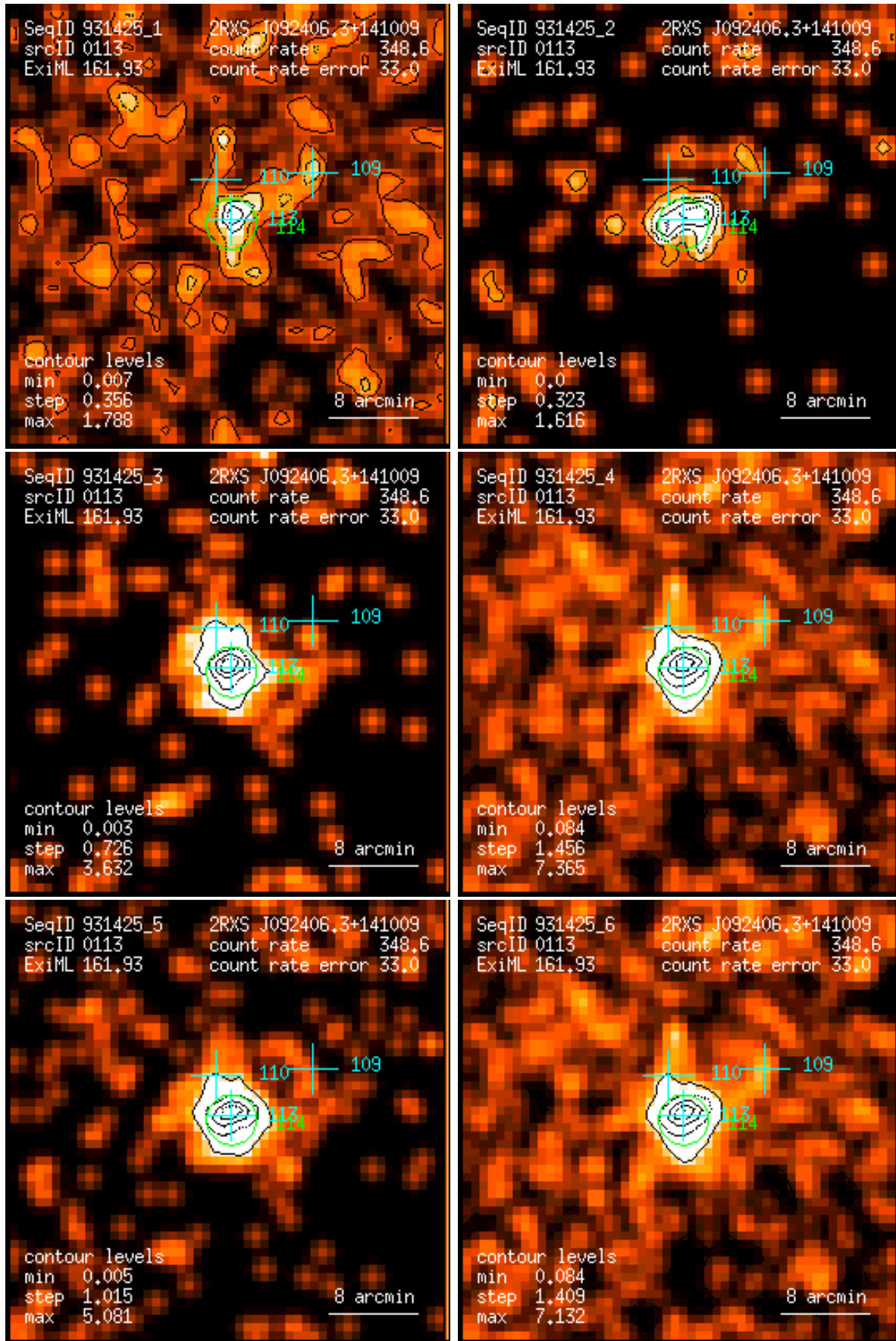
Figure 113: RASS 931425: detection 0113: band rate images, Gaussian filter: (1) PSPC channels 11 – 41, (2) 52 – 90, (3) 91 – 201, (4) 11 – 235, (5) 52 – 201, (6) 11 – 201. Broad band rates in counts/ks. Band rate contour levels in counts/ks/arcmin 2 .
