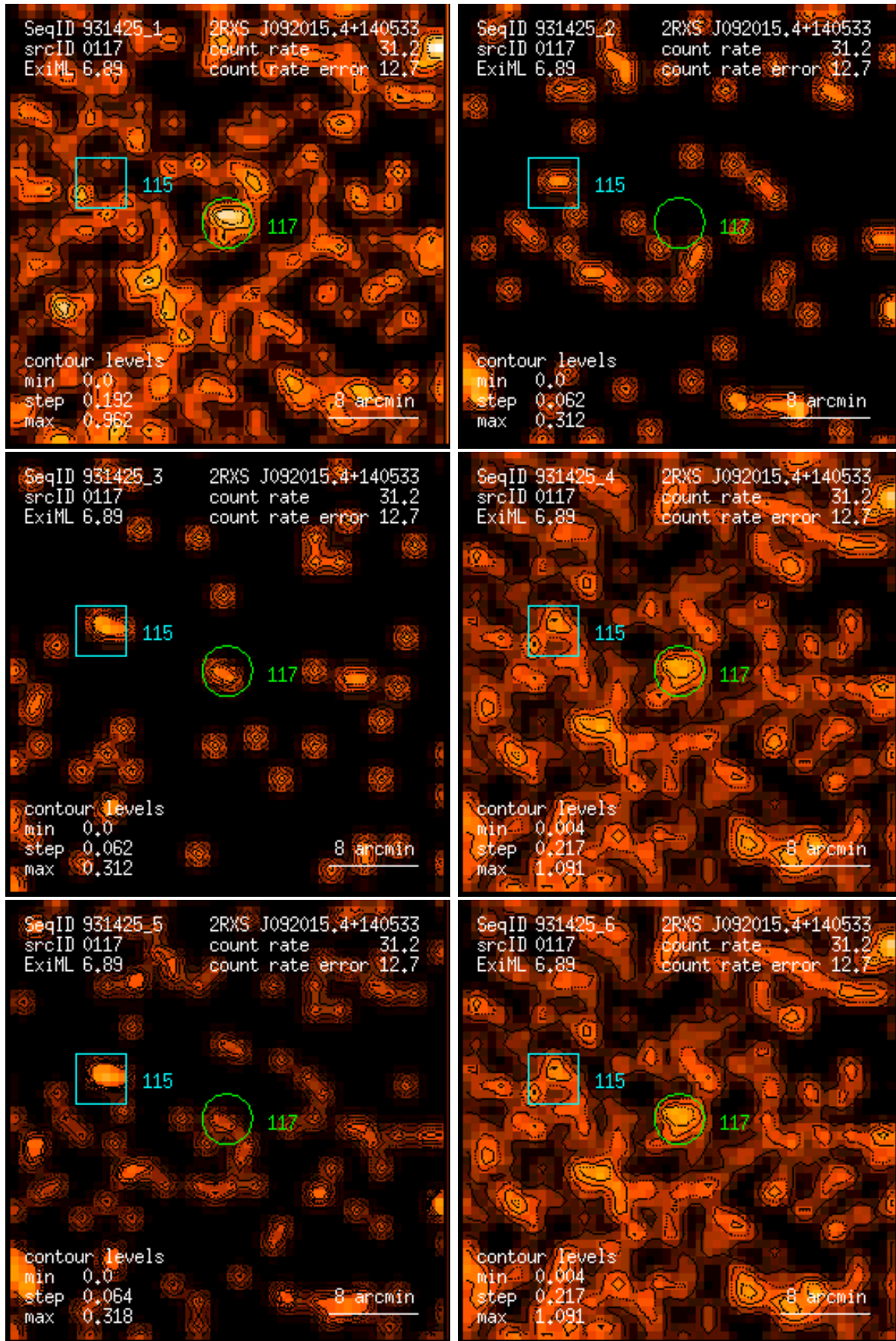
Figure 117: RASS 931425: detection 0117: band rate images, Gaussian filter: (1) PSPC channels 11 – 41, (2) 52 – 90, (3) 91 – 201, (4) 11 – 235, (5) 52 – 201, (6) 11 – 201. Broad band rates in counts/ks. Band rate contour levels in counts/ks/arcmin 2 .
