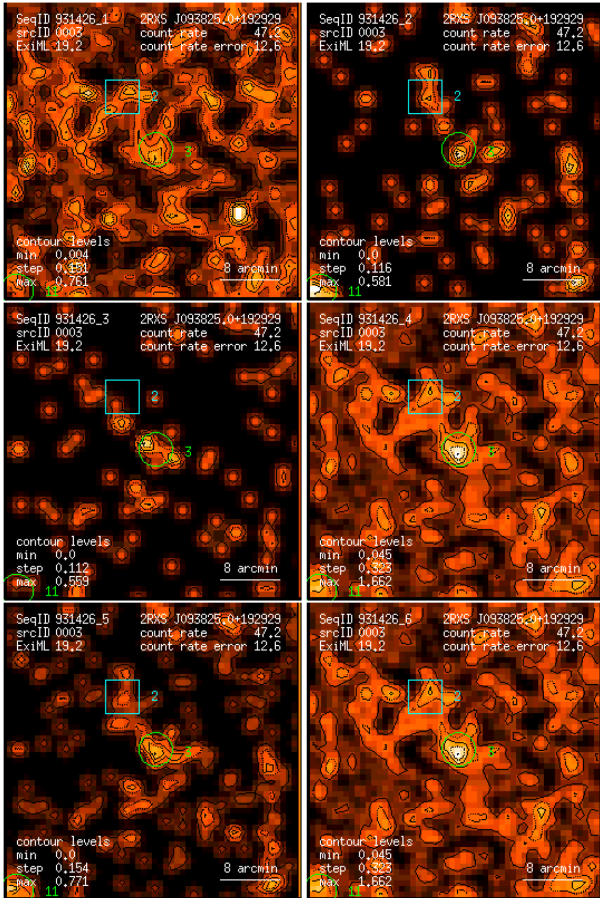
Figure 3: RASS 931426: detection 0003: band rate images, Gaussian filter: (1) PSPC channels 11 – 41, (2) 52 – 90, (3) 91 – 201, (4) 11 – 235, (5) 52 – 201, (6) 11 – 201. Broad band rates in counts/ks. Band rate contour levels in counts/ks/arcmin 2 .
