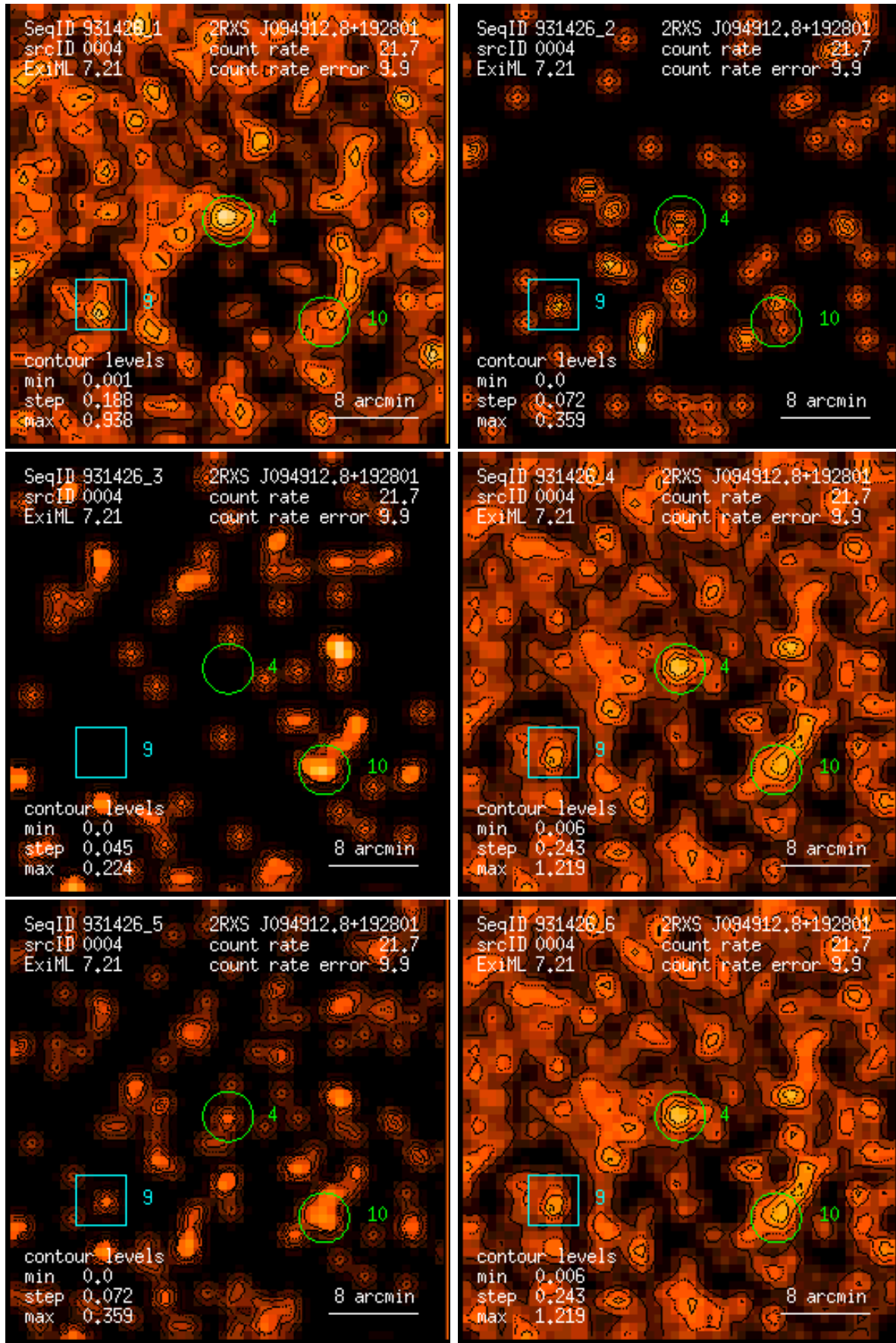
Figure 4: RASS 931426: detection 0004: band rate images, Gaussian filter: (1) PSPC channels 11 – 41, (2) 52 – 90, (3) 91 – 201, (4) 11 – 235, (5) 52 – 201, (6) 11 – 201. Broad band rates in counts/ks. Band rate contour levels in counts/ks/arcmin 2 .
