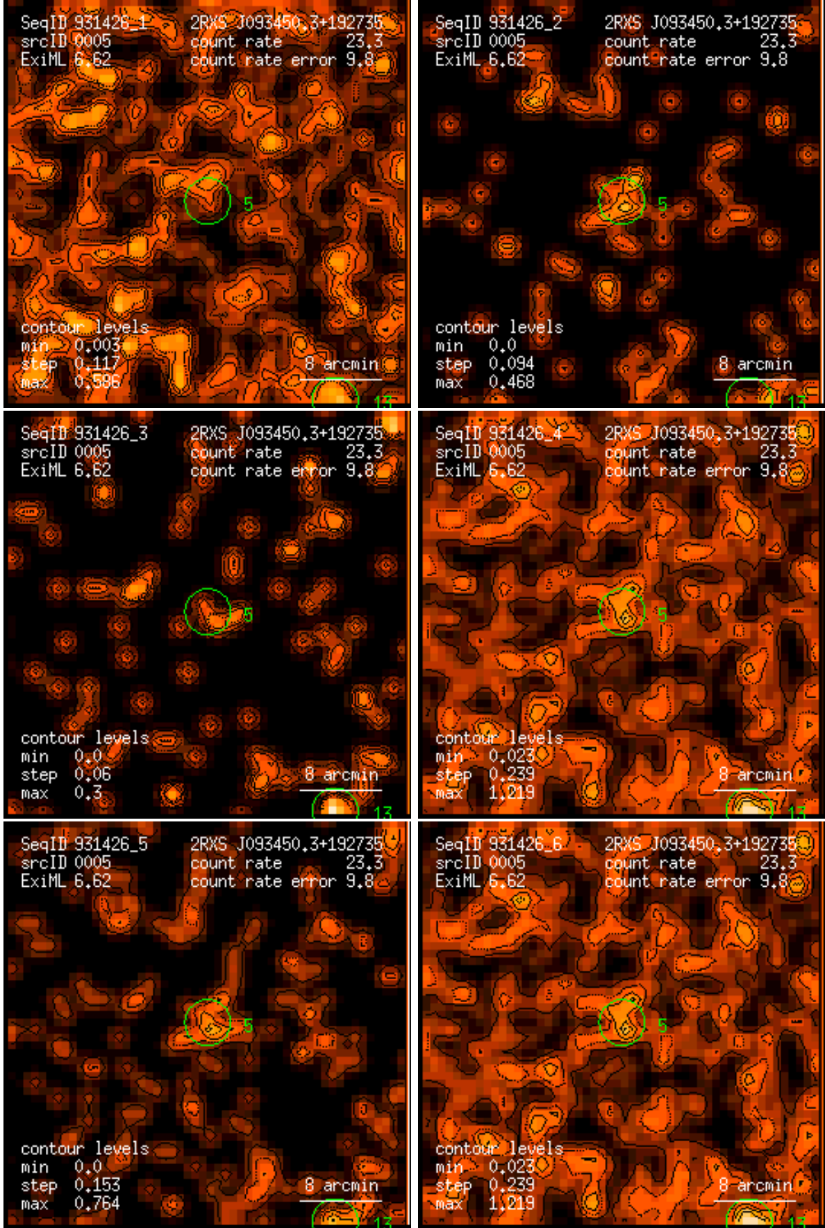
Figure 5: RASS 931426: detection 0005: band rate images, Gaussian filter: (1) PSPC channels 11 – 41, (2) 52 – 90, (3) 91 – 201, (4) 11 – 235, (5) 52 – 201, (6) 11 – 201. Broad band rates in counts/ks. Band rate contour levels in counts/ks/arcmin 2 .
