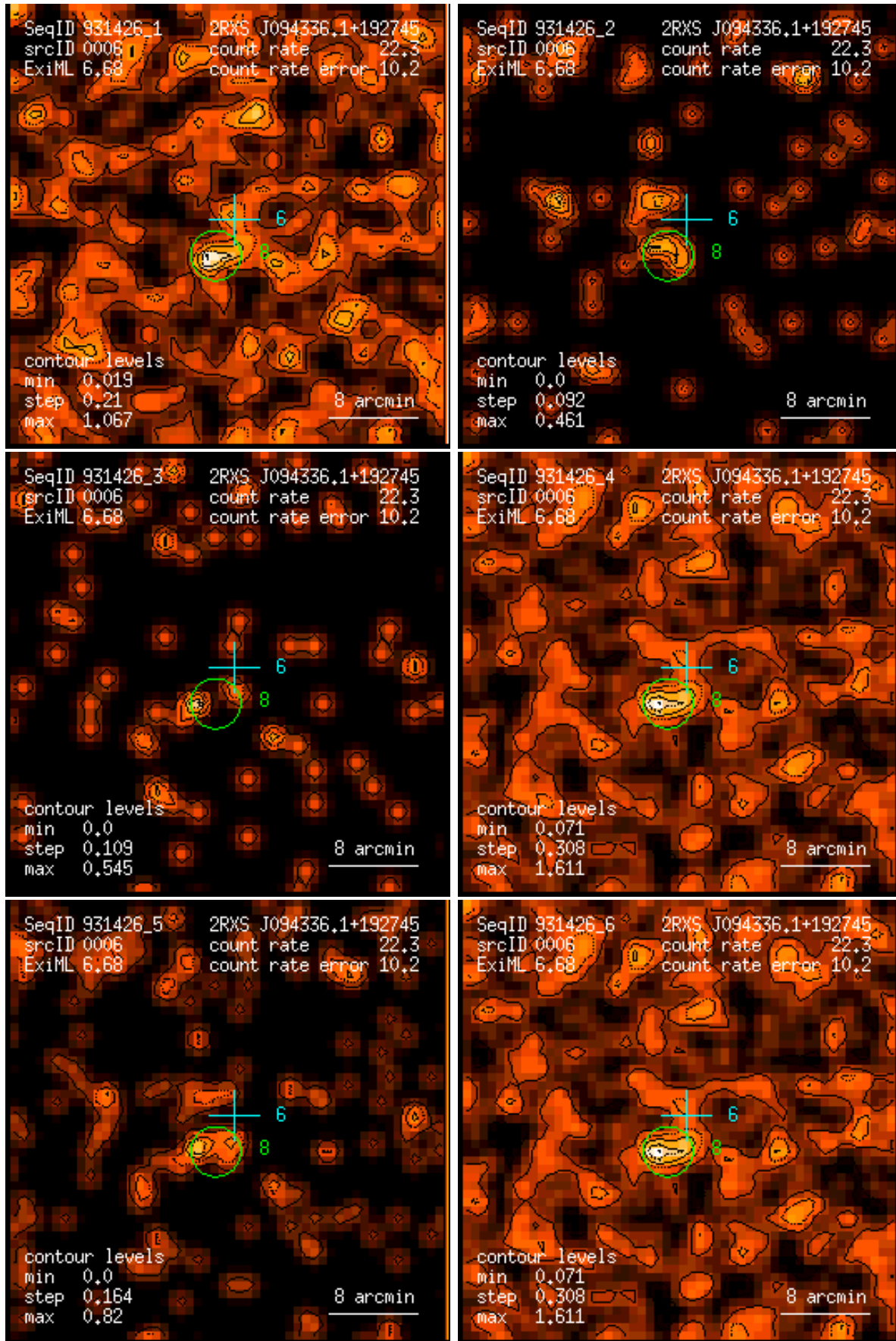
Figure 6: RASS 931426: detection 0006: band rate images, Gaussian filter: (1) PSPC channels 11 – 41, (2) 52 – 90, (3) 91 – 201, (4) 11 – 235, (5) 52 – 201, (6) 11 – 201. Broad band rates in counts/ks. Band rate contour levels in counts/ks/arcmin 2 .
