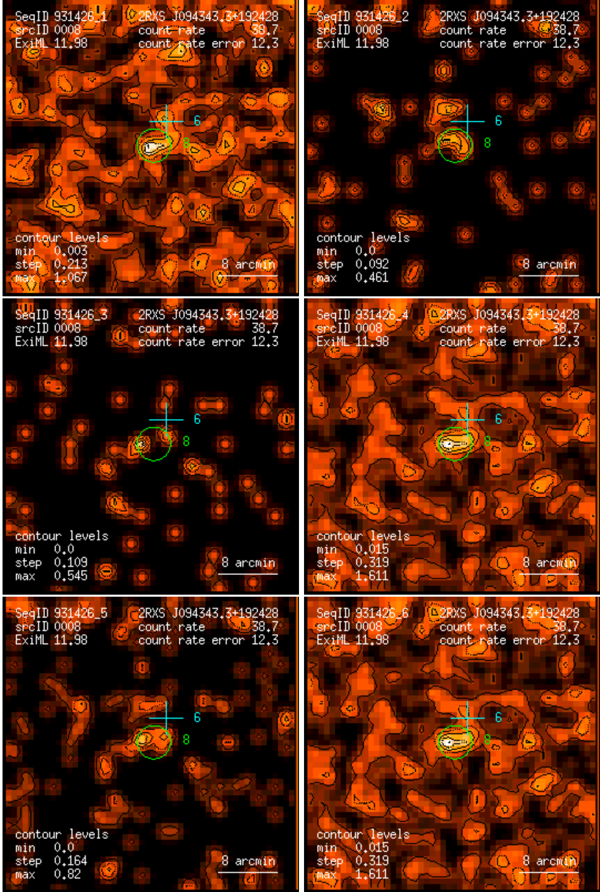
Figure 8: RASS 931426: detection 0008: band rate images, Gaussian filter: (1) PSPC channels 11 – 41, (2) 52 – 90, (3) 91 – 201, (4) 11 – 235, (5) 52 – 201, (6) 11 – 201. Broad band rates in counts/ks. Band rate contour levels in counts/ks/arcmin 2 .
