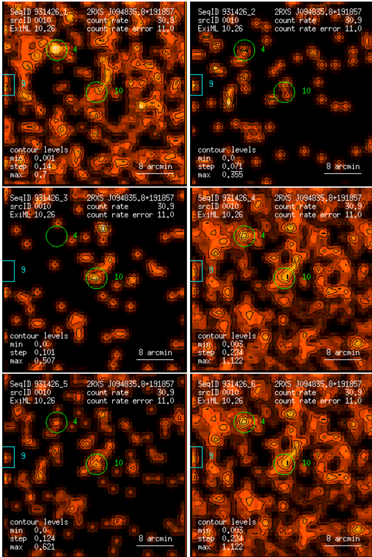
Figure 10: RASS 931426: detection 0010: band rate images, Gaussian filter: (1) PSPC channels 11 – 41, (2) 52 – 90, (3) 91 – 201, (4) 11 – 235, (5) 52 – 201, (6) 11 – 201. Broad band rates in counts/ks. Band rate contour levels in counts/ks/arcmin 2 .
