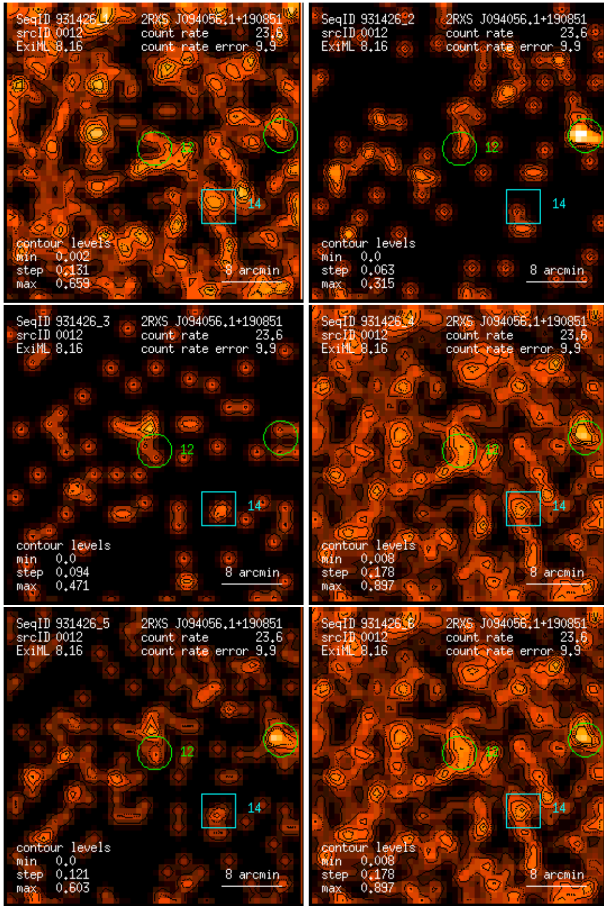
Figure 12: RASS 931426: detection 0012: band rate images, Gaussian filter: (1) PSPC channels 11 – 41, (2) 52 – 90, (3) 91 – 201, (4) 11 – 235, (5) 52 – 201, (6) 11 – 201. Broad band rates in counts/ks. Band rate contour levels in counts/ks/arcmin 2 .
