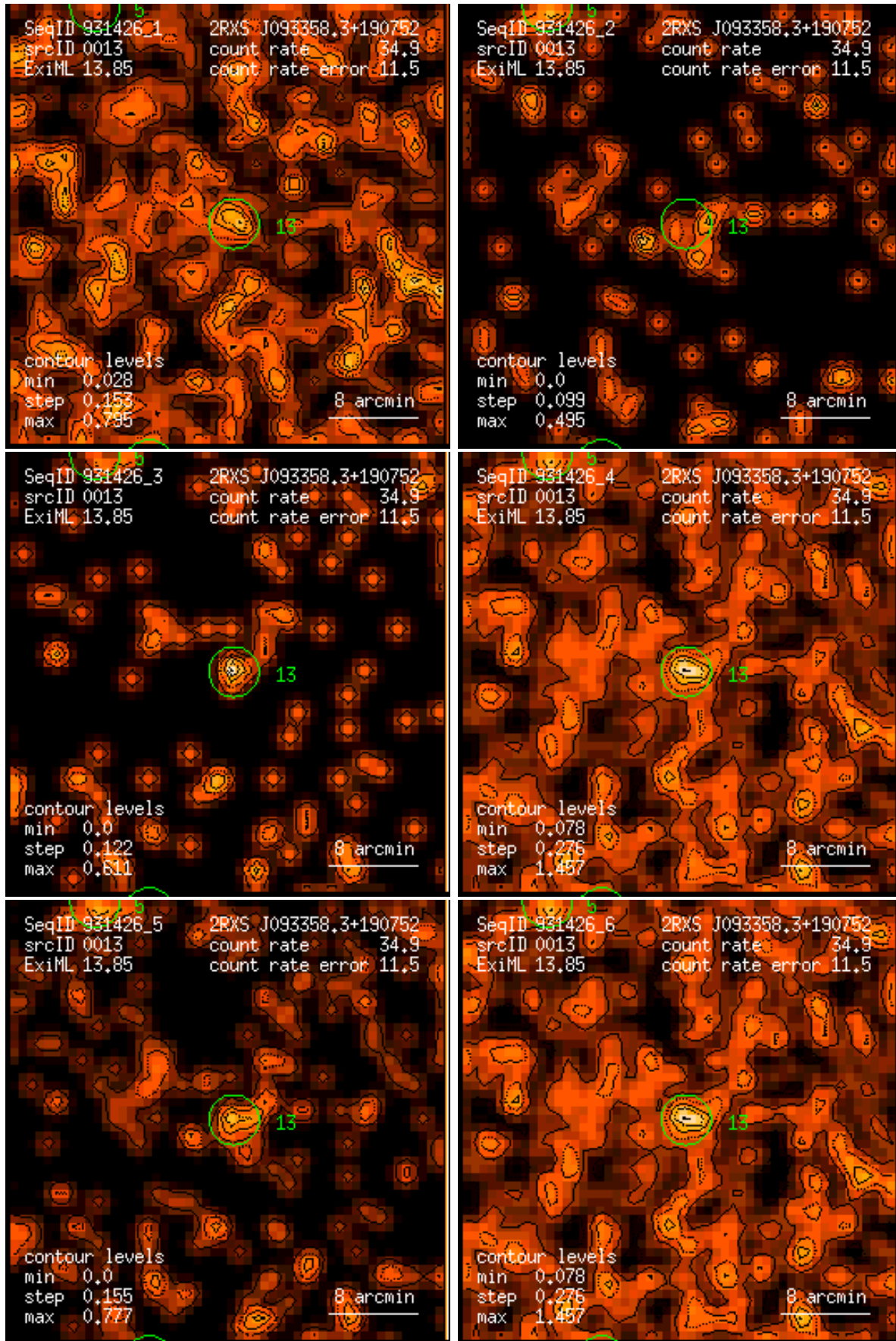
Figure 13: RASS 931426: detection 0013: band rate images, Gaussian filter: (1) PSPC channels 11 – 41, (2) 52 – 90, (3) 91 – 201, (4) 11 – 235, (5) 52 – 201, (6) 11 – 201. Broad band rates in counts/ks. Band rate contour levels in counts/ks/arcmin 2 .
