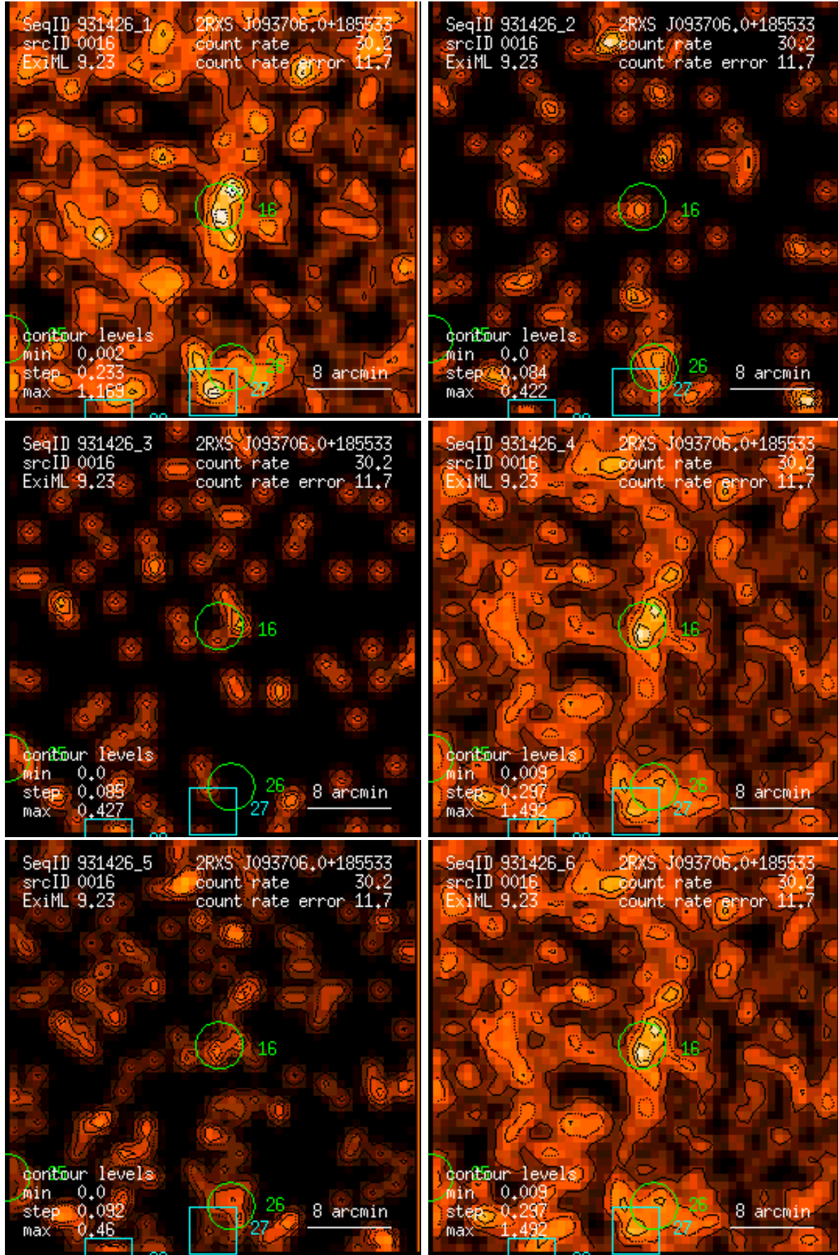
Figure 16: RASS 931426: detection 0016: band rate images, Gaussian filter: (1) PSPC channels 11 – 41, (2) 52 – 90, (3) 91 – 201, (4) 11 – 235, (5) 52 – 201, (6) 11 – 201. Broad band rates in counts/ks. Band rate contour levels in counts/ks/arcmin 2 .
