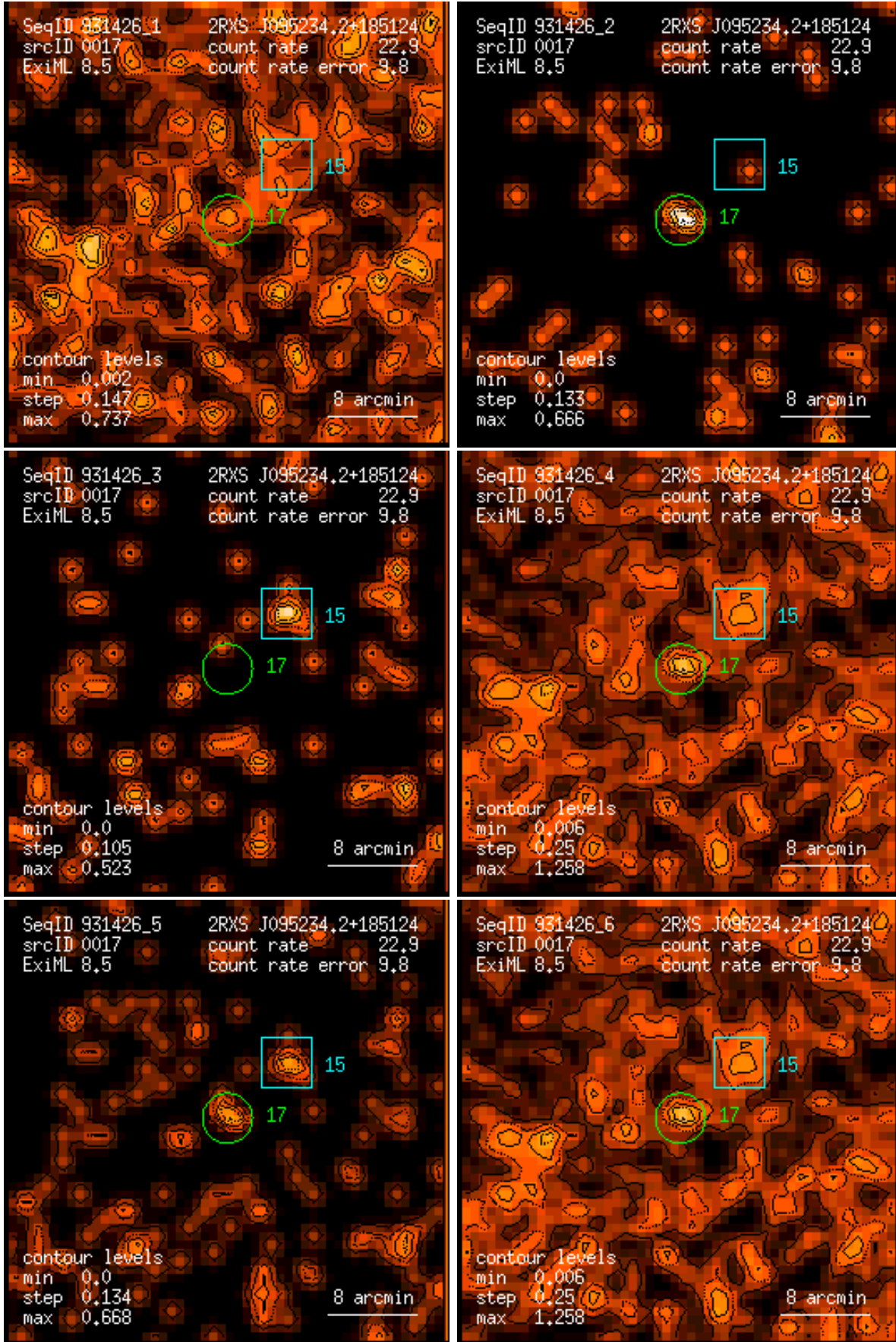
Figure 17: RASS 931426: detection 0017: band rate images, Gaussian filter: (1) PSPC channels 11 – 41, (2) 52 – 90, (3) 91 – 201, (4) 11 – 235, (5) 52 – 201, (6) 11 – 201. Broad band rates in counts/ks. Band rate contour levels in counts/ks/arcmin 2 .
