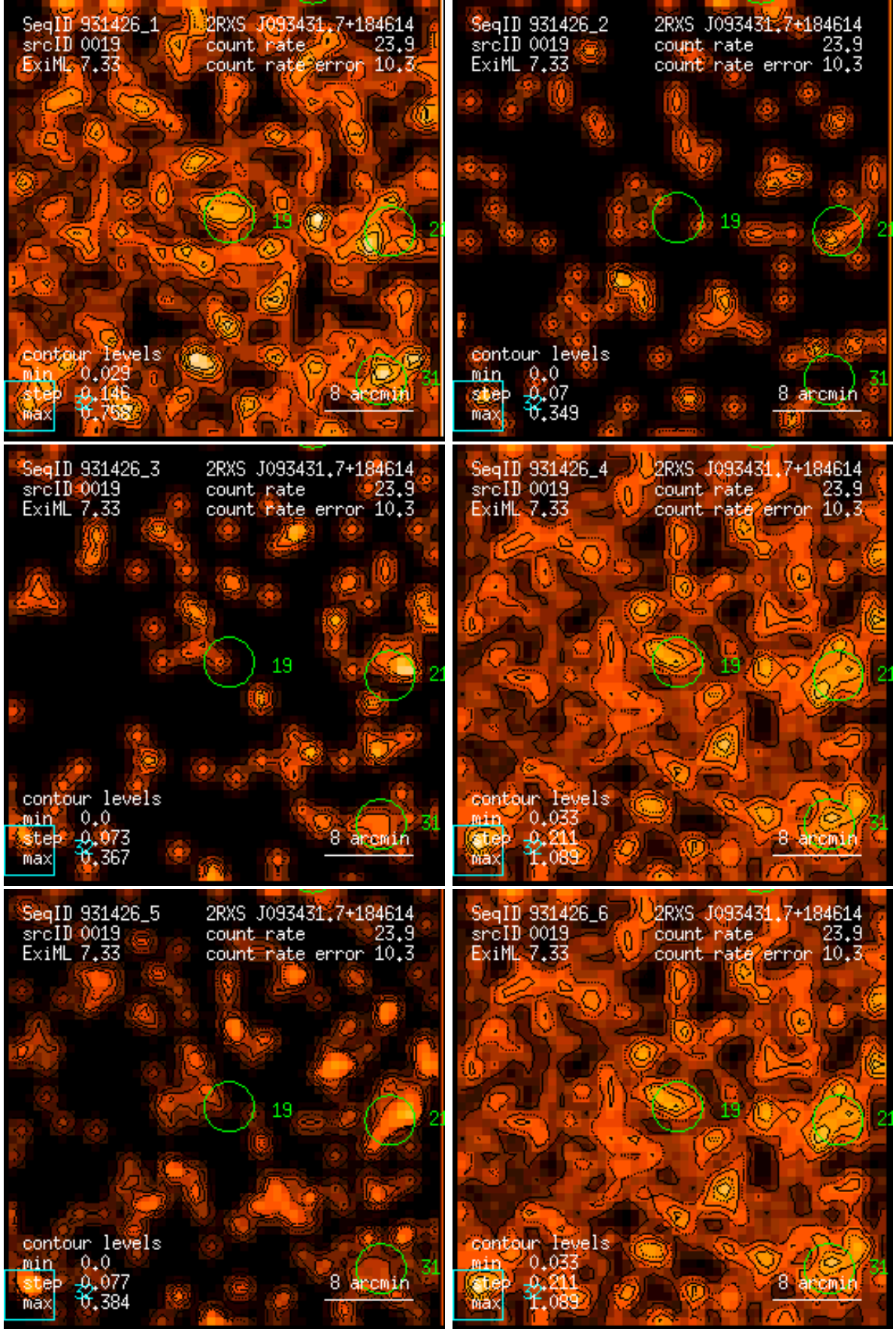
Figure 19: RASS 931426: detection 0019: band rate images, Gaussian filter: (1) PSPC channels 11 – 41, (2) 52 – 90, (3) 91 – 201, (4) 11 – 235, (5) 52 – 201, (6) 11 – 201. Broad band rates in counts/ks. Band rate contour levels in counts/ks/arcmin 2 .
