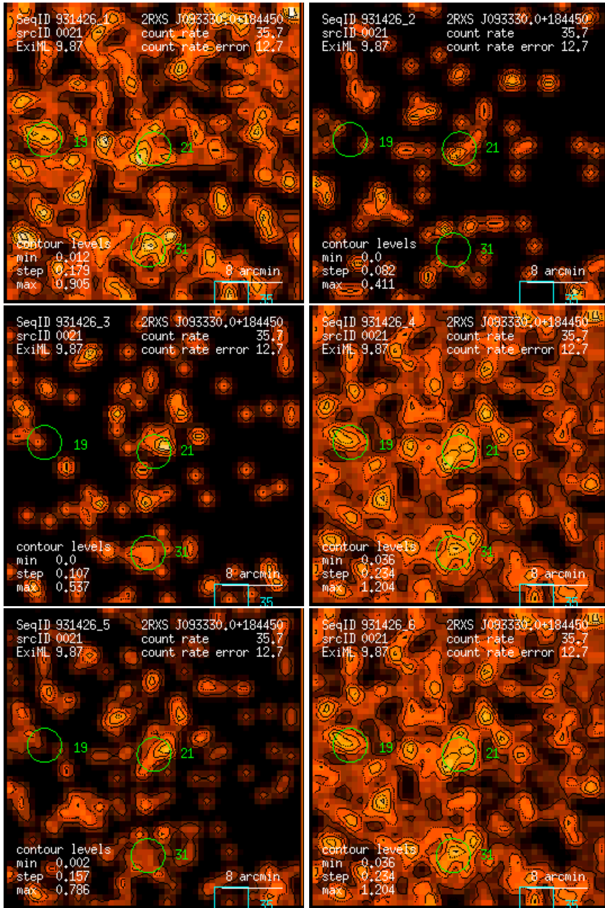
Figure 21: RASS 931426: detection 0021: band rate images, Gaussian filter: (1) PSPC channels 11 – 41, (2) 52 – 90, (3) 91 – 201, (4) 11 – 235, (5) 52 – 201, (6) 11 – 201. Broad band rates in counts/ks. Band rate contour levels in counts/ks/arcmin 2 .
