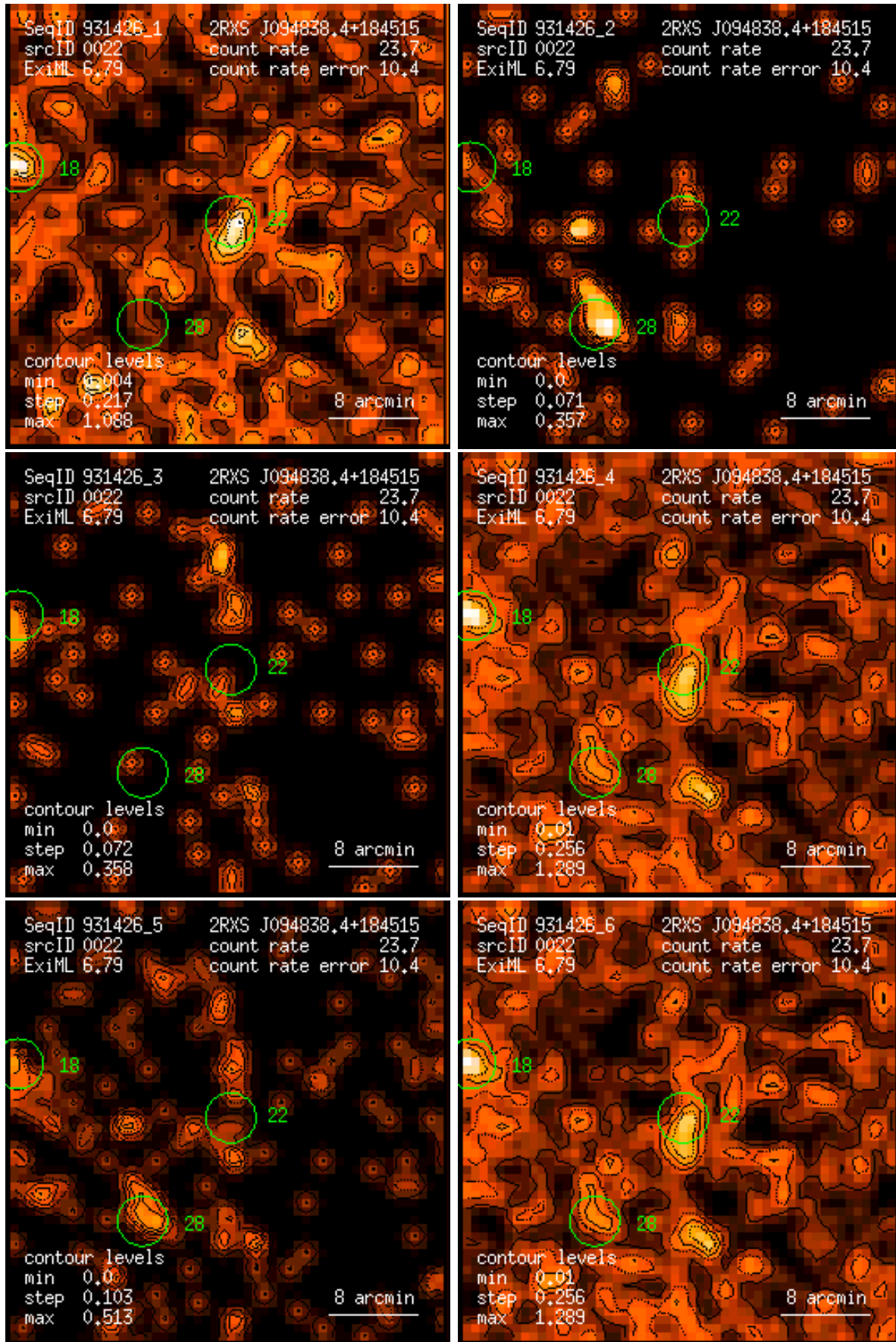
Figure 22: RASS 931426: detection 0022: band rate images, Gaussian filter: (1) PSPC channels 11 – 41, (2) 52 – 90, (3) 91 – 201, (4) 11 – 235, (5) 52 – 201, (6) 11 – 201. Broad band rates in counts/ks. Band rate contour levels in counts/ks/arcmin 2 .
