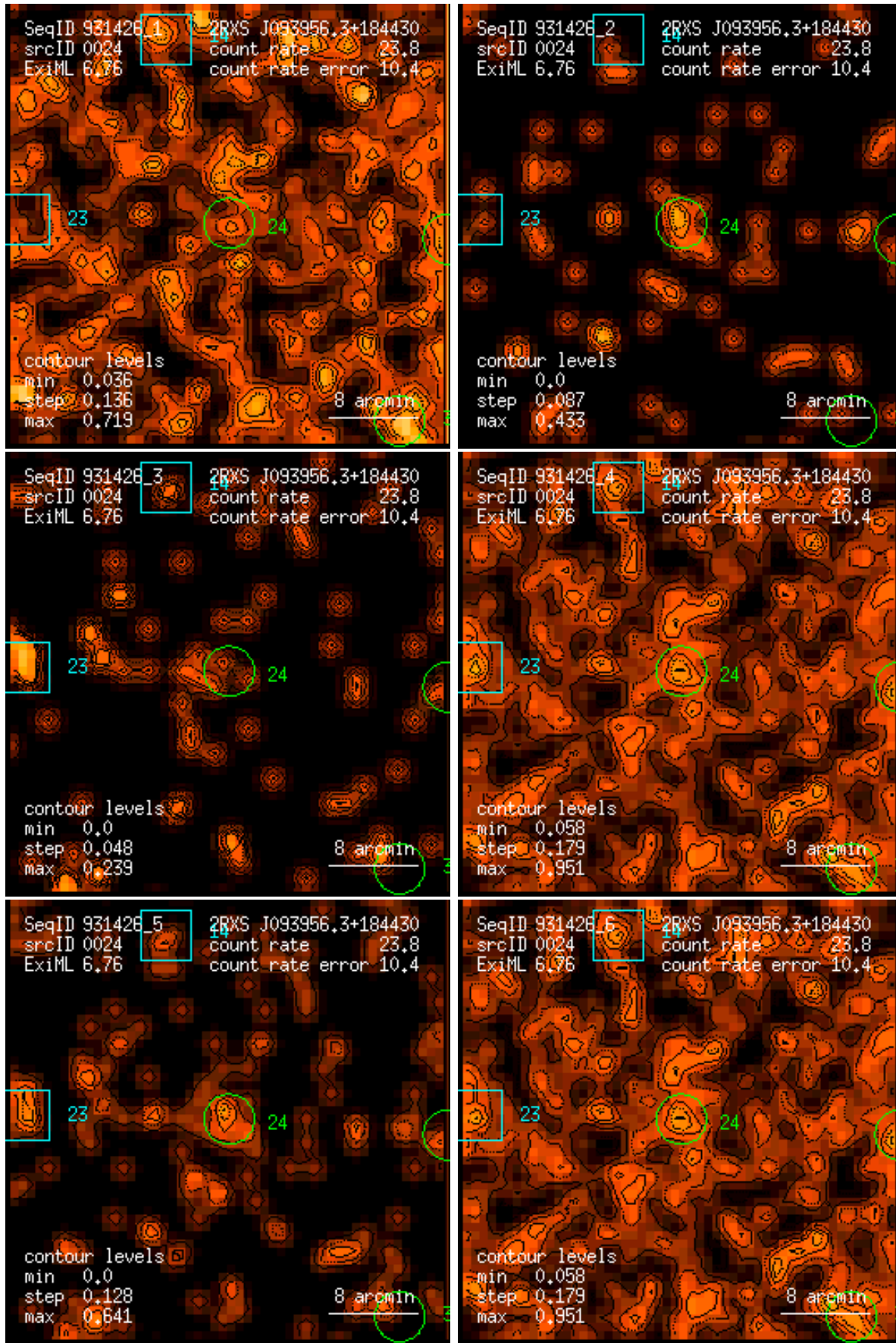
Figure 24: RASS 931426: detection 0024: band rate images, Gaussian filter: (1) PSPC channels 11 – 41, (2) 52 – 90, (3) 91 – 201, (4) 11 – 235, (5) 52 – 201, (6) 11 – 201. Broad band rates in counts/ks. Band rate contour levels in counts/ks/arcmin 2 .
