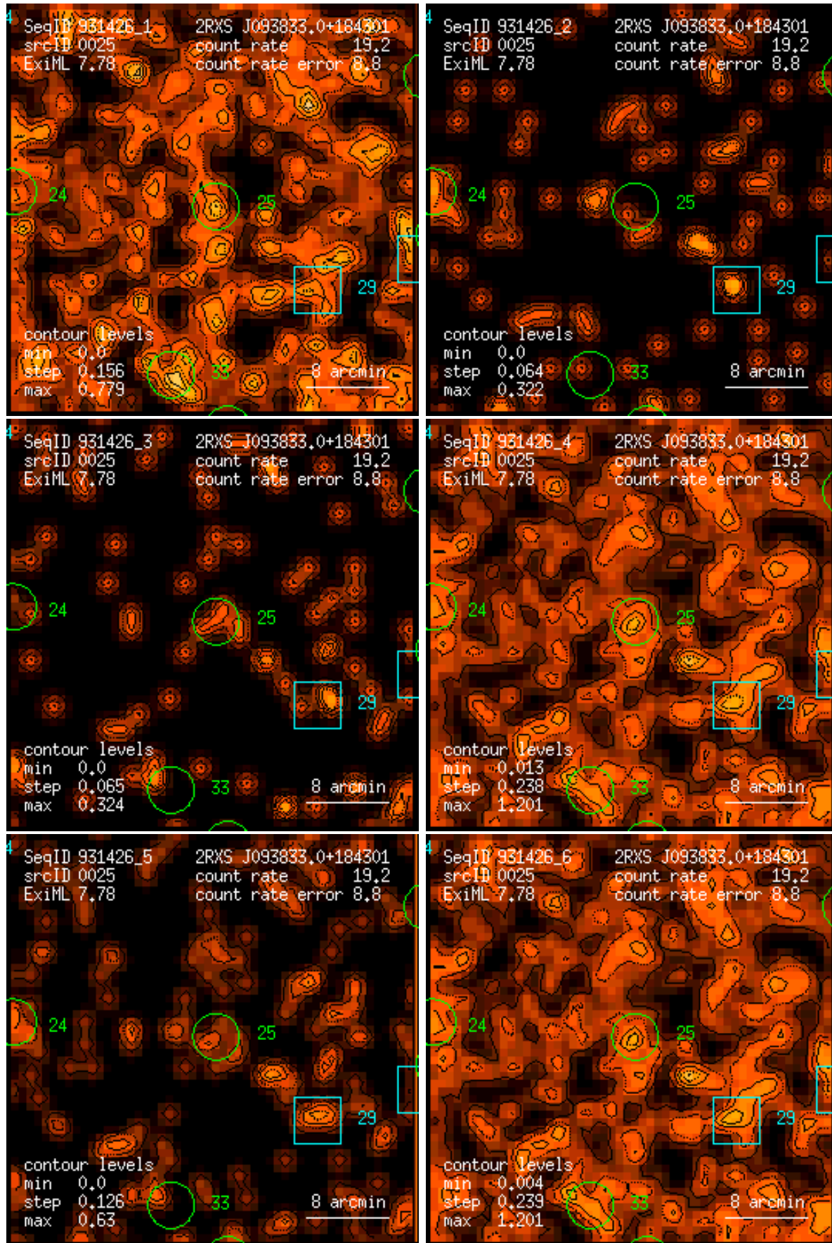
Figure 25: RASS 931426: detection 0025: band rate images, Gaussian filter: (1) PSPC channels 11 – 41, (2) 52 – 90, (3) 91 – 201, (4) 11 – 235, (5) 52 – 201, (6) 11 – 201. Broad band rates in counts/ks. Band rate contour levels in counts/ks/arcmin 2 .
