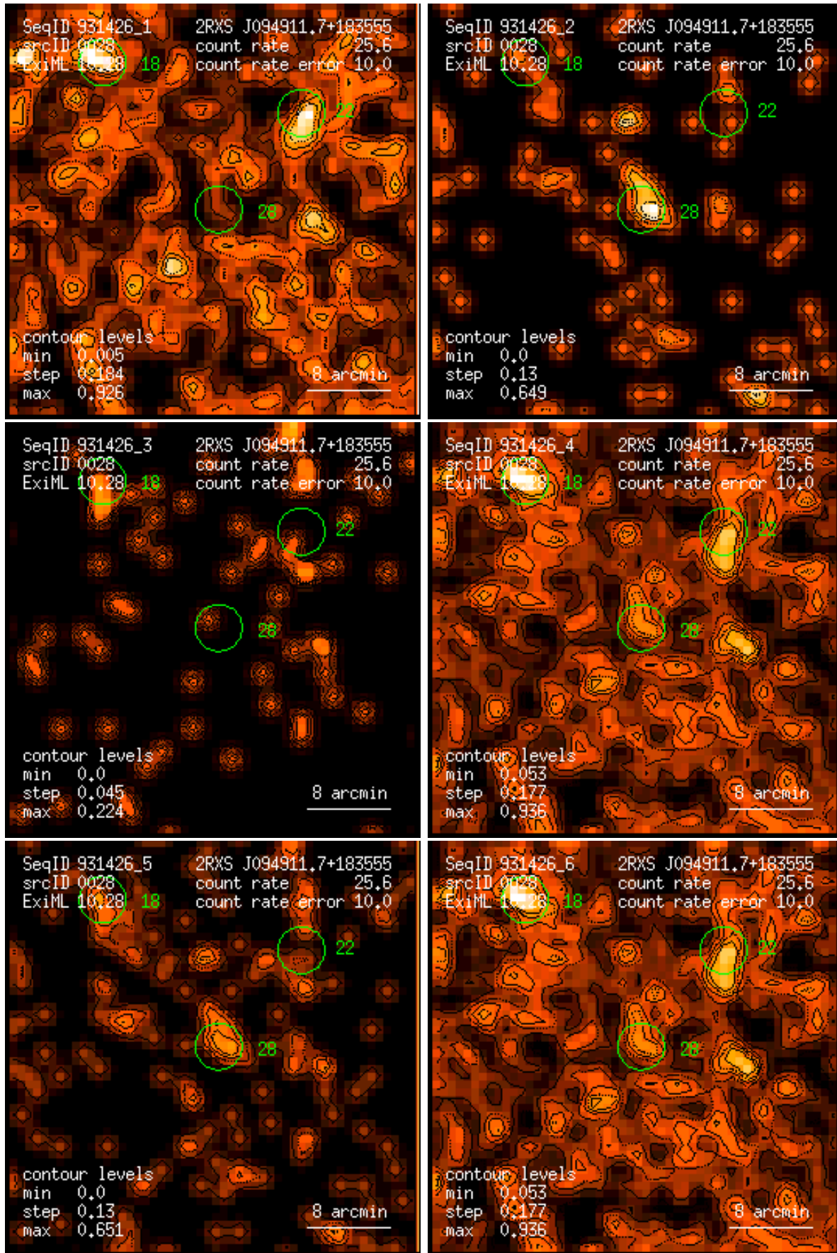
Figure 28: RASS 931426: detection 0028: band rate images, Gaussian filter: (1) PSPC channels 11 – 41, (2) 52 – 90, (3) 91 – 201, (4) 11 – 235, (5) 52 – 201, (6) 11 – 201. Broad band rates in counts/ks. Band rate contour levels in counts/ks/arcmin 2 .
