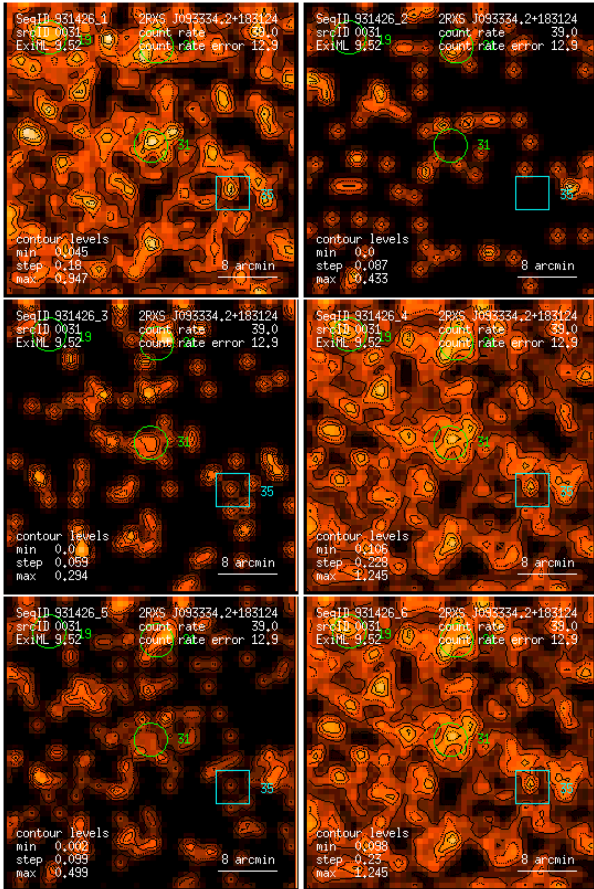
Figure 31: RASS 931426: detection 0031: band rate images, Gaussian filter: (1) PSPC channels 11 – 41, (2) 52 – 90, (3) 91 – 201, (4) 11 – 235, (5) 52 – 201, (6) 11 – 201. Broad band rates in counts/ks. Band rate contour levels in counts/ks/arcmin 2 .
