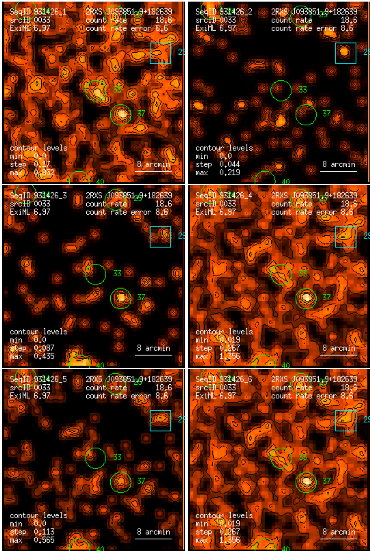
Figure 33: RASS 931426: detection 0033: band rate images, Gaussian filter: (1) PSPC channels 11 – 41, (2) 52 – 90, (3) 91 – 201, (4) 11 – 235, (5) 52 – 201, (6) 11 – 201. Broad band rates in counts/ks. Band rate contour levels in counts/ks/arcmin 2 .
