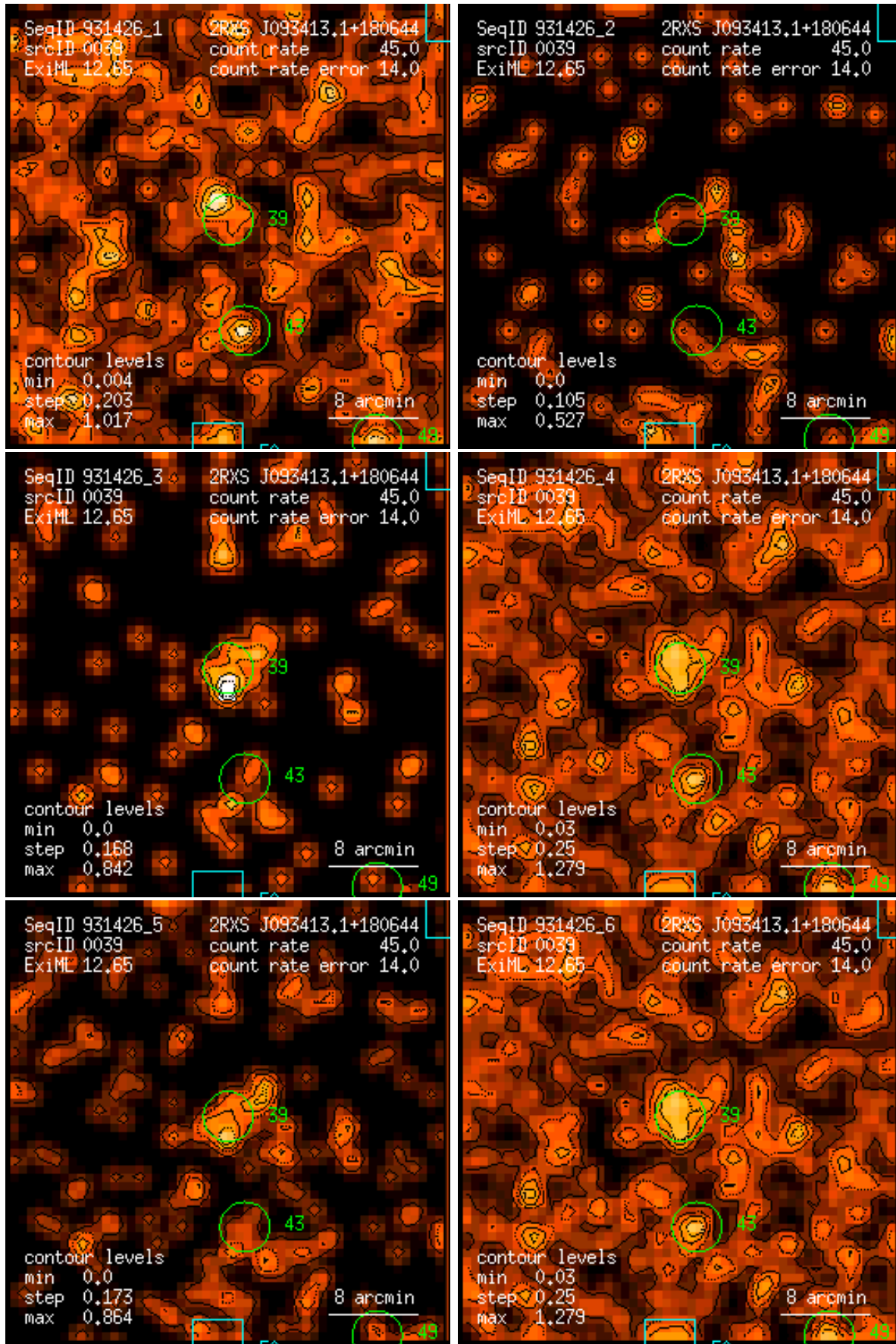
Figure 39: RASS 931426: detection 0039: band rate images, Gaussian filter: (1) PSPC channels 11 – 41, (2) 52 – 90, (3) 91 – 201, (4) 11 – 235, (5) 52 – 201, (6) 11 – 201. Broad band rates in counts/ks. Band rate contour levels in counts/ks/arcmin 2 .
