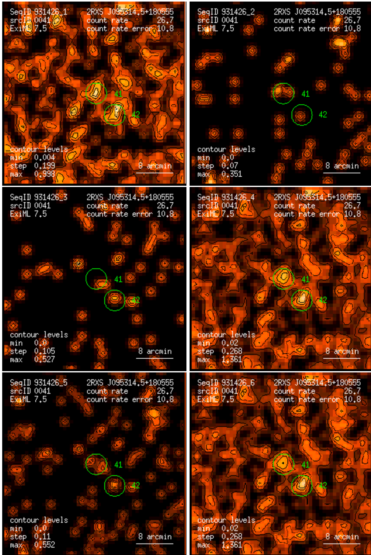
Figure 41: RASS 931426: detection 0041: band rate images, Gaussian filter: (1) PSPC channels 11 – 41, (2) 52 – 90, (3) 91 – 201, (4) 11 – 235, (5) 52 – 201, (6) 11 – 201. Broad band rates in counts/ks. Band rate contour levels in counts/ks/arcmin 2 .
