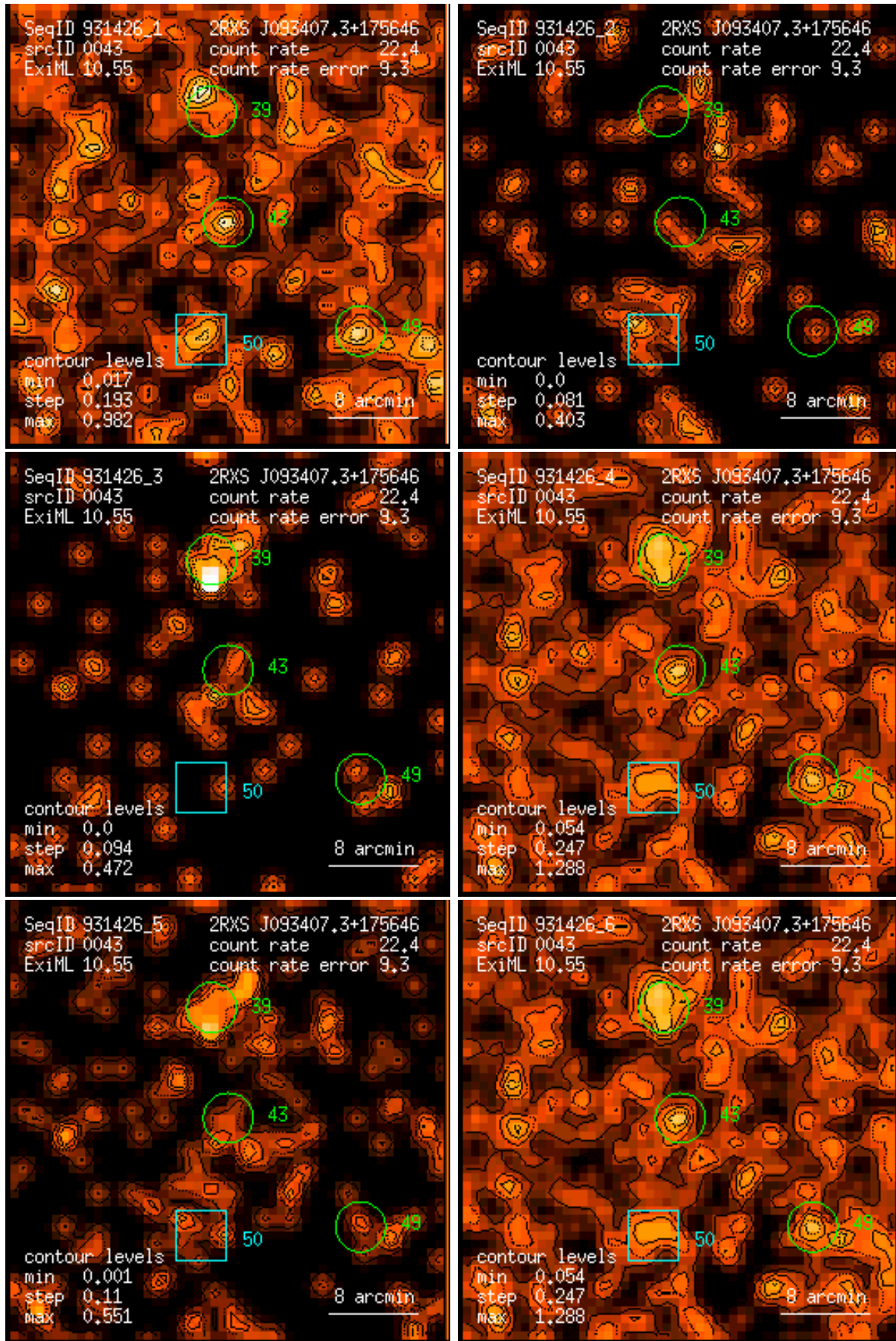
Figure 43: RASS 931426: detection 0043: band rate images, Gaussian filter: (1) PSPC channels 11 – 41, (2) 52 – 90, (3) 91 – 201, (4) 11 – 235, (5) 52 – 201, (6) 11 – 201. Broad band rates in counts/ks. Band rate contour levels in counts/ks/arcmin 2 .
