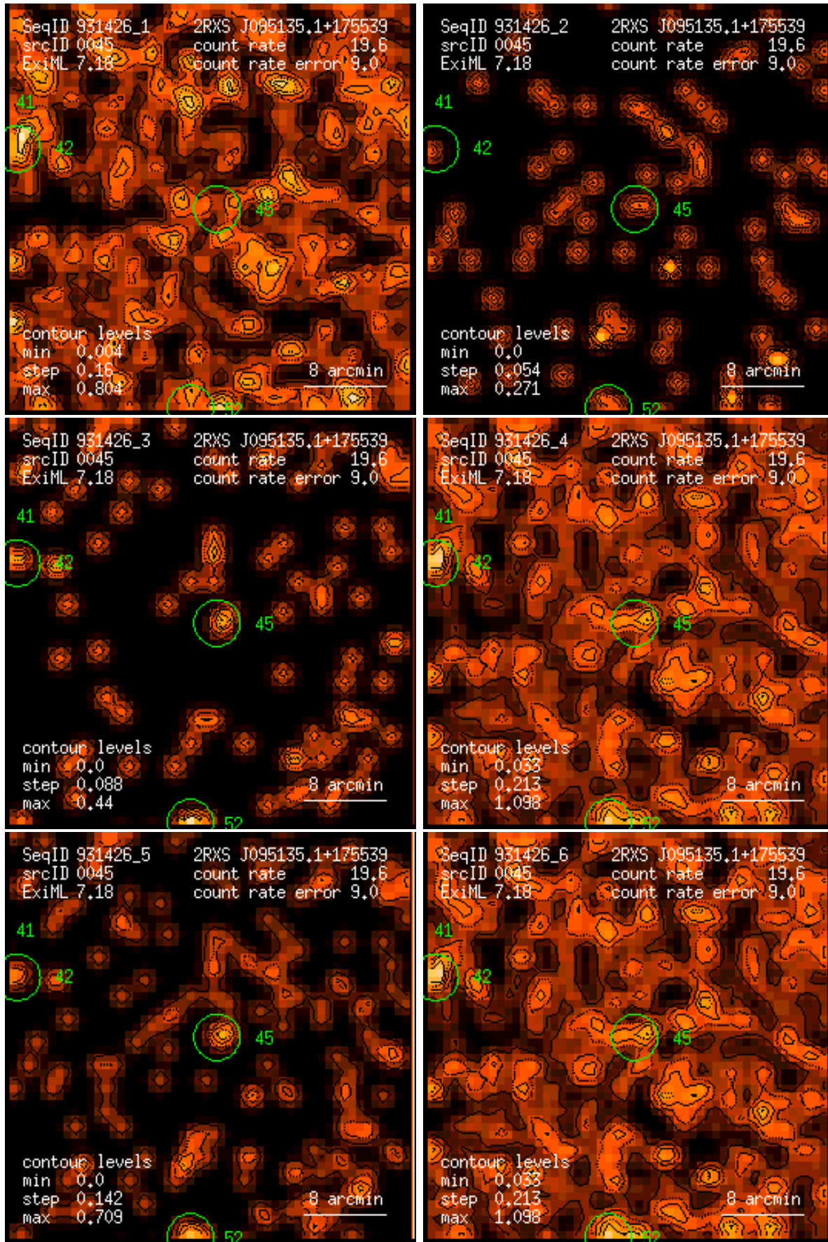
Figure 45: RASS 931426: detection 0045: band rate images, Gaussian filter: (1) PSPC channels 11 – 41, (2) 52 – 90, (3) 91 – 201, (4) 11 – 235, (5) 52 – 201, (6) 11 – 201. Broad band rates in counts/ks. Band rate contour levels in counts/ks/arcmin 2 .
