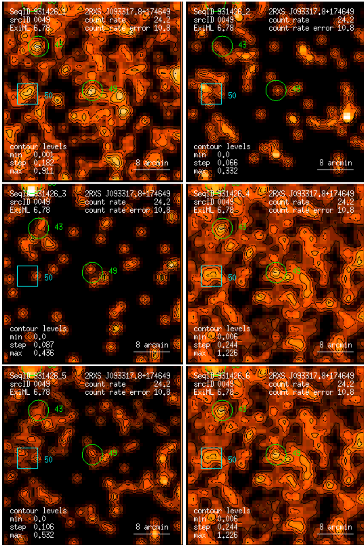
Figure 49: RASS 931426: detection 0049: band rate images, Gaussian filter: (1) PSPC channels 11 – 41, (2) 52 – 90, (3) 91 – 201, (4) 11 – 235, (5) 52 – 201, (6) 11 – 201. Broad band rates in counts/ks. Band rate contour levels in counts/ks/arcmin 2 .
