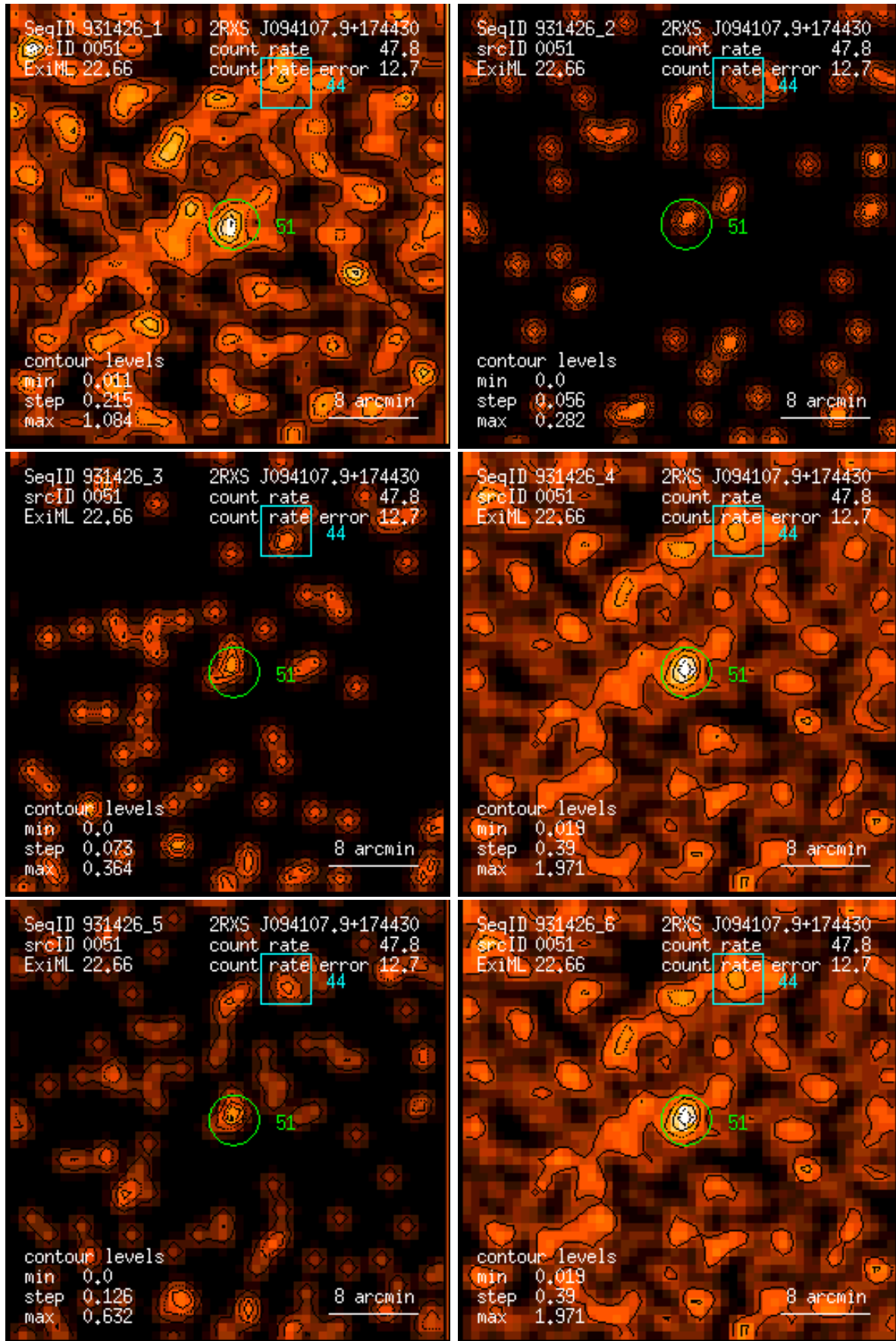
Figure 51: RASS 931426: detection 0051: band rate images, Gaussian filter: (1) PSPC channels 11 – 41, (2) 52 – 90, (3) 91 – 201, (4) 11 – 235, (5) 52 – 201, (6) 11 – 201. Broad band rates in counts/ks. Band rate contour levels in counts/ks/arcmin 2 .
