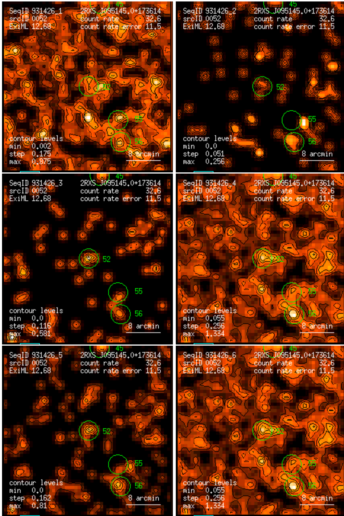
Figure 52: RASS 931426: detection 0052: band rate images, Gaussian filter: (1) PSPC channels 11 – 41, (2) 52 – 90, (3) 91 – 201, (4) 11 – 235, (5) 52 – 201, (6) 11 – 201. Broad band rates in counts/ks. Band rate contour levels in counts/ks/arcmin 2 .
