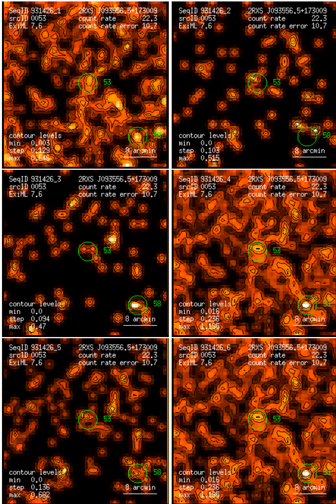
Figure 53: RASS 931426: detection 0053: band rate images, Gaussian filter: (1) PSPC channels 11 – 41, (2) 52 – 90, (3) 91 – 201, (4) 11 – 235, (5) 52 – 201, (6) 11 – 201. Broad band rates in counts/ks. Band rate contour levels in counts/ks/arcmin 2 .
