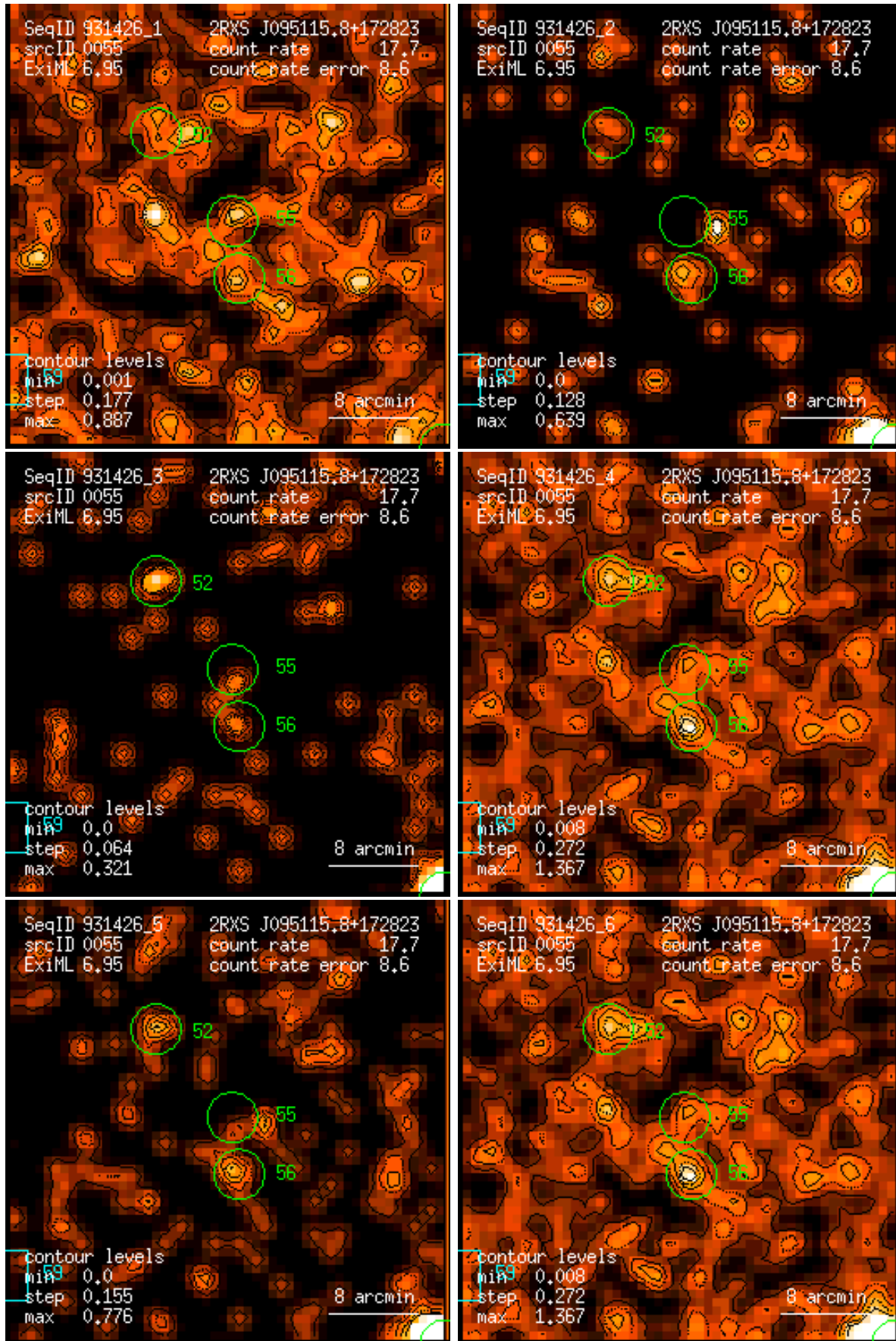
Figure 55: RASS 931426: detection 0055: band rate images, Gaussian filter: (1) PSPC channels 11 – 41, (2) 52 – 90, (3) 91 – 201, (4) 11 – 235, (5) 52 – 201, (6) 11 – 201. Broad band rates in counts/ks. Band rate contour levels in counts/ks/arcmin 2 .
