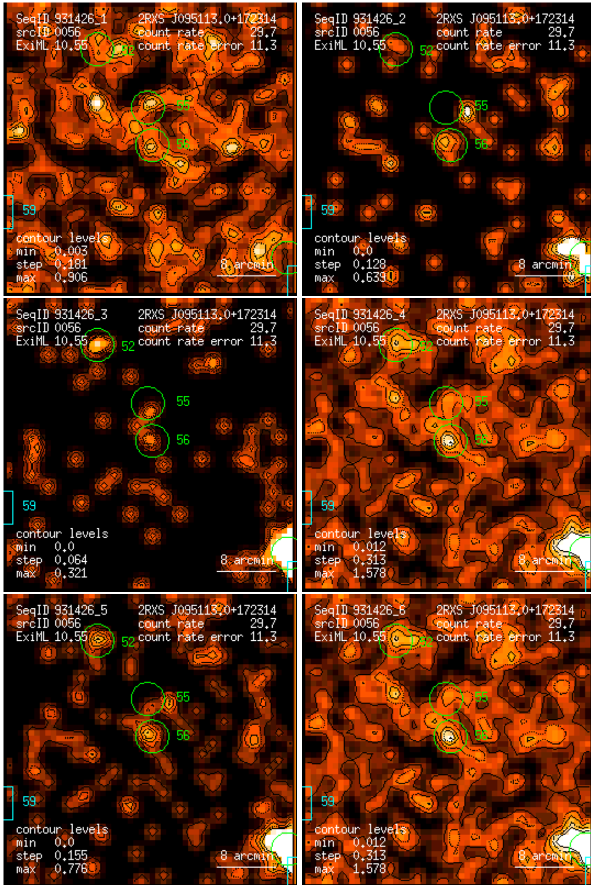
Figure 56: RASS 931426: detection 0056: band rate images, Gaussian filter: (1) PSPC channels 11 – 41, (2) 52 – 90, (3) 91 – 201, (4) 11 – 235, (5) 52 – 201, (6) 11 – 201. Broad band rates in counts/ks. Band rate contour levels in counts/ks/arcmin 2 .
