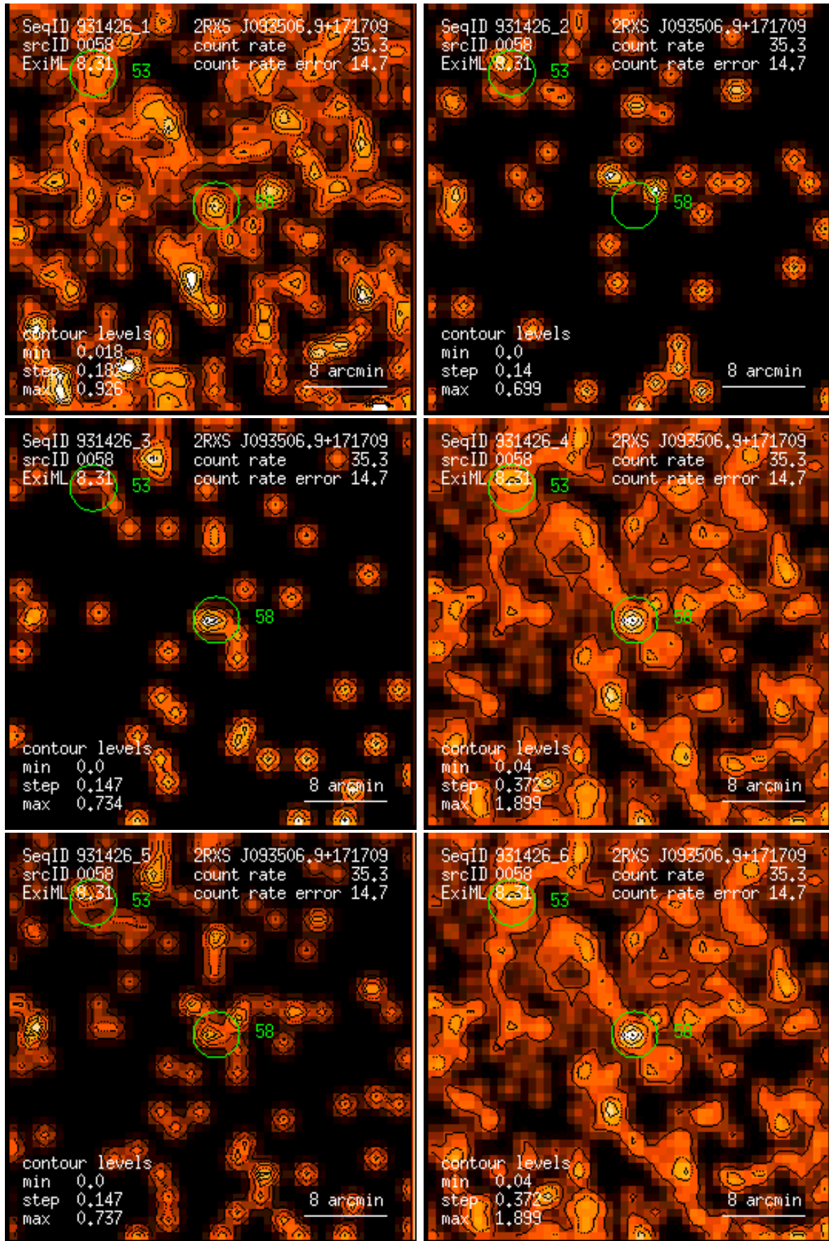
Figure 58: RASS 931426: detection 0058: band rate images, Gaussian filter: (1) PSPC channels 11 – 41, (2) 52 – 90, (3) 91 – 201, (4) 11 – 235, (5) 52 – 201, (6) 11 – 201. Broad band rates in counts/ks. Band rate contour levels in counts/ks/arcmin 2 .
